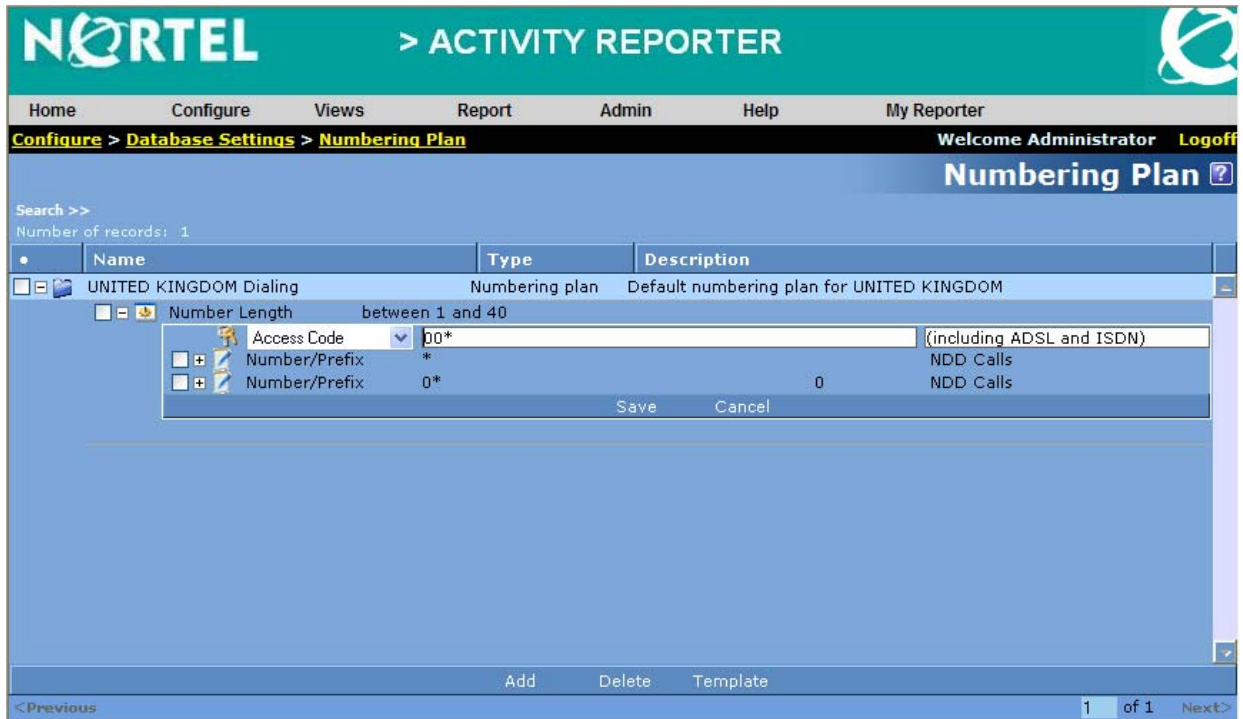
Figure 38: Editing International Numbering Plan Access Codes
