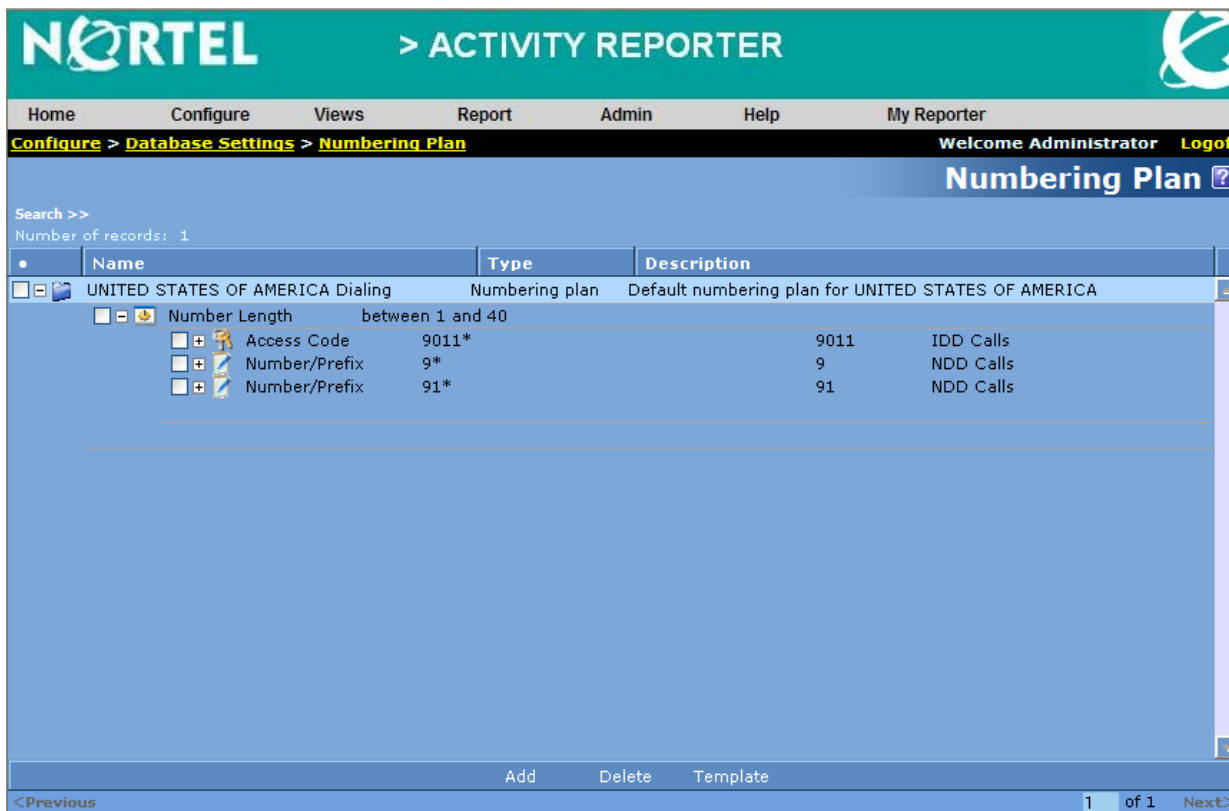
Figure 34: Modified NANP Number Plan Access Codes/Number Prefixes
