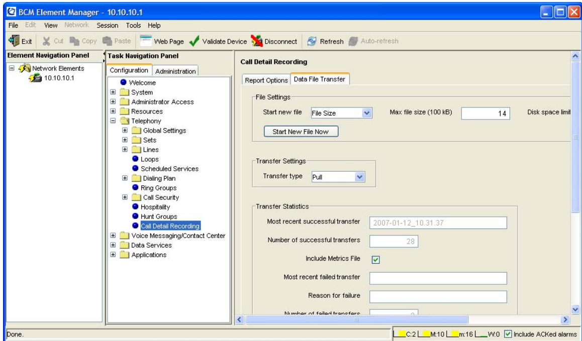
Figure 4: BCM Call Detail Recording Data File Transfer Options
