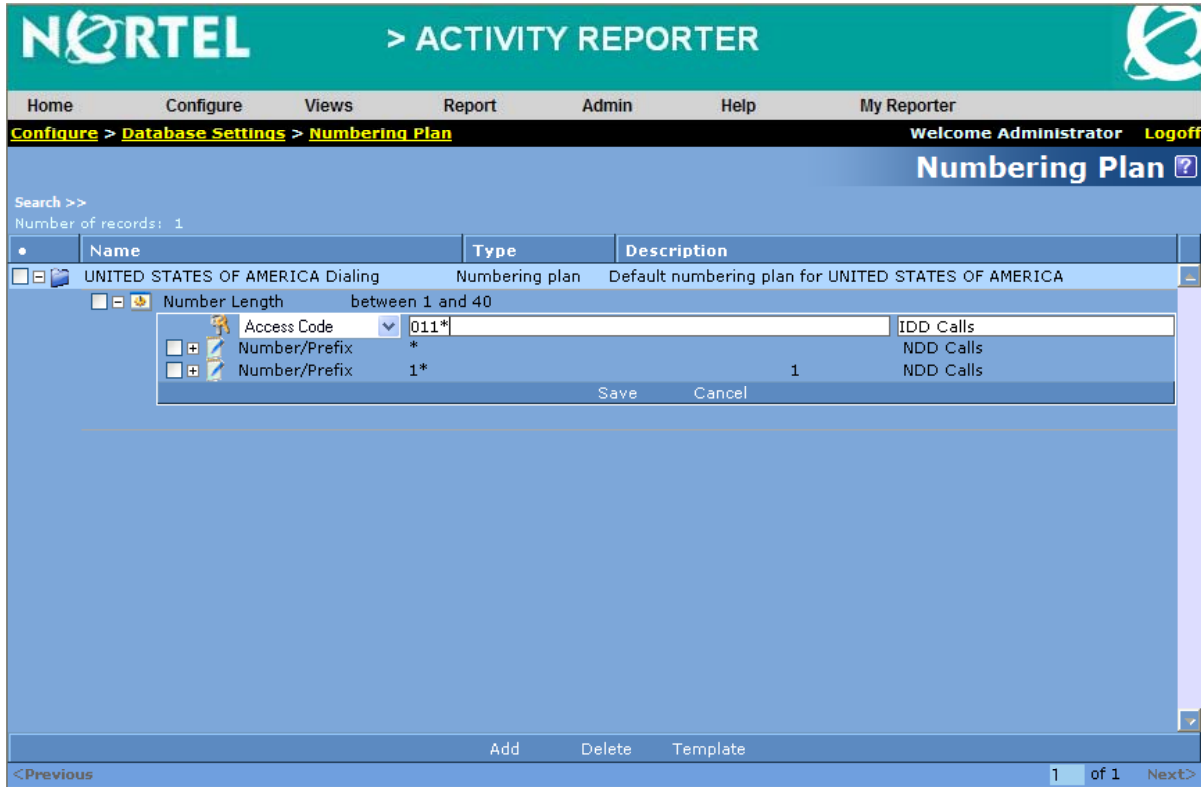
Figure 32: Editing NANP Numbering Plan Access Code
