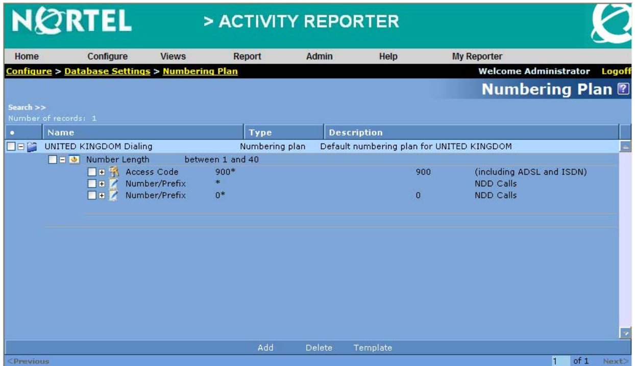
Figure 39: Modified International Numbering Plan Access Codes
