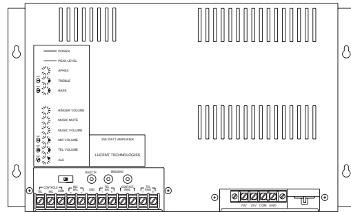
Figure 1: Telephone Paging Amplifier
