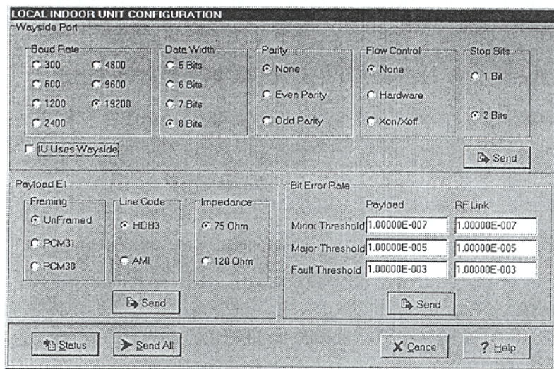
Figure 14. Indoor Unit: Typical E1 Configuration Screen.
