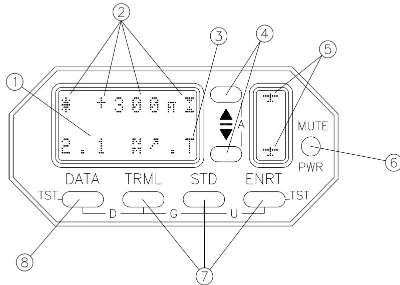
Figure 5. ½ 3ATI Traffic Display After Traffic Acquisition
