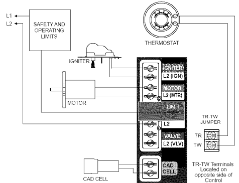
Figure 8 – 7505B (for replacement of R7184B)
