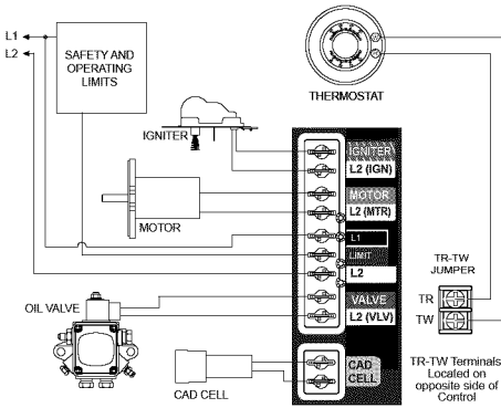
Figure 9 – 7505P (for replacement of R7184P)
