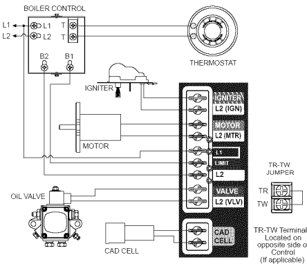
Figure 5 – 7505P (for replacement of R7184P)
