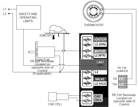
Figure 6 – 7505A (for replacement of R8184G)
