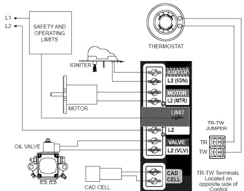
Figure 8 – 7505B (for replacement of R7184B)
