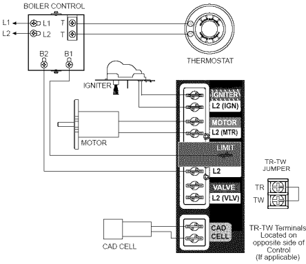
Figure 4 – 7505B (for replacement of R7184B)
