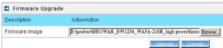
Figure 282 – Firmware Upgrade
