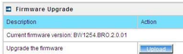
Figure 126 – Firmware Upgrade
