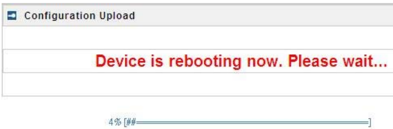
Figure 277 – Configuration Upload/Restore - 3
