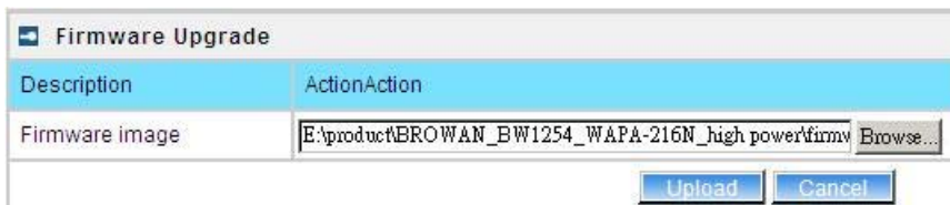
Figure 127 – Firmware Upgrade
