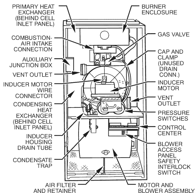
Fig. 2 - Variable-Speed Model in Upflow Orientation
