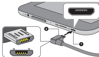
Figure 4-2 Connecting an Micro-USB cable
