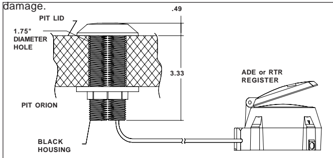
Figure 4 - Identification - Pit ORION Transmitter
