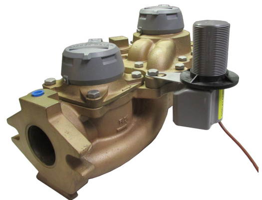
Figure 38: Endpoint connected to meter with bracket
