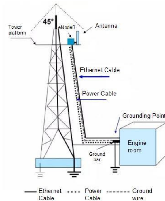
Figure 2-1 Grounding and Lightning Protection
