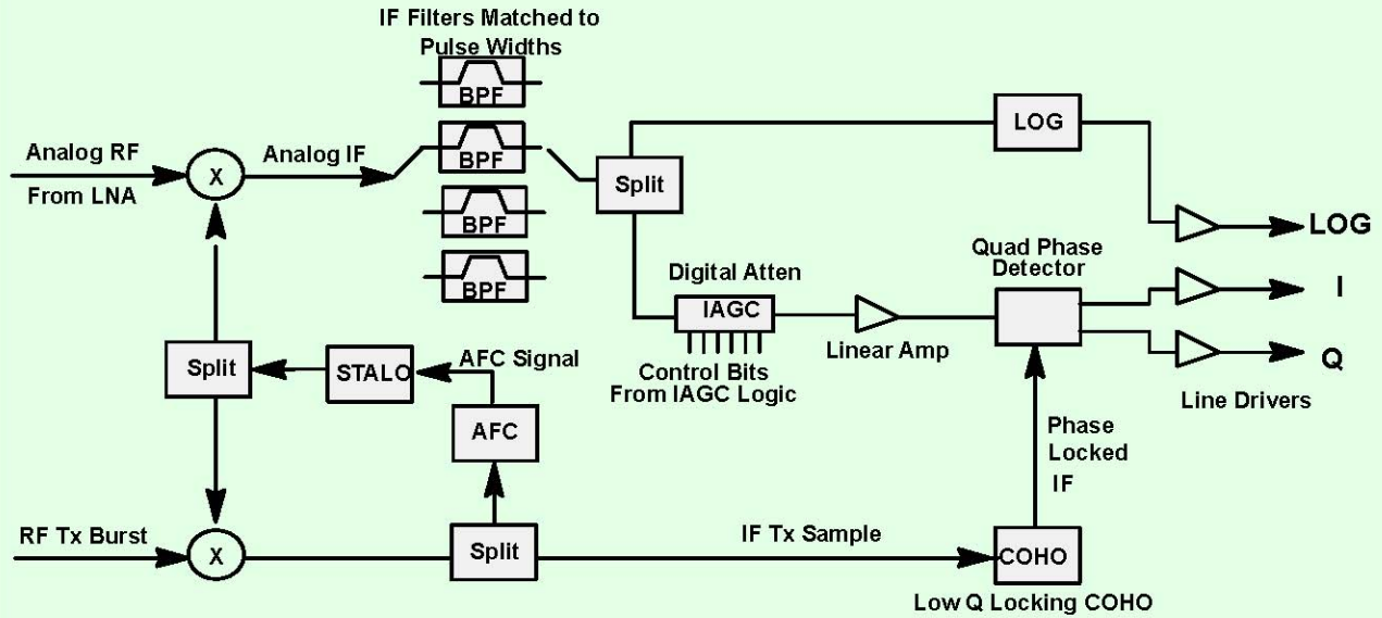
Figure 1-1: Analog vs Digital Receiver for Magnetron Systems Classic Analog Receiver for Magnetron
