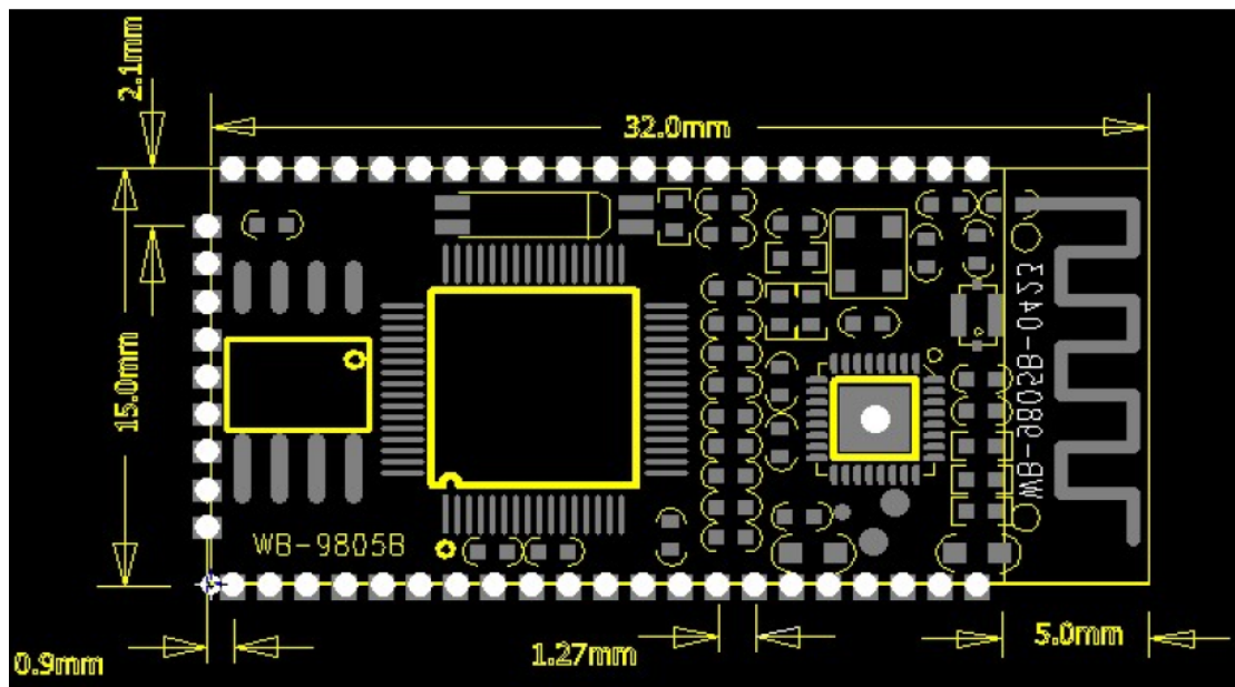
WB-9805B PCB
