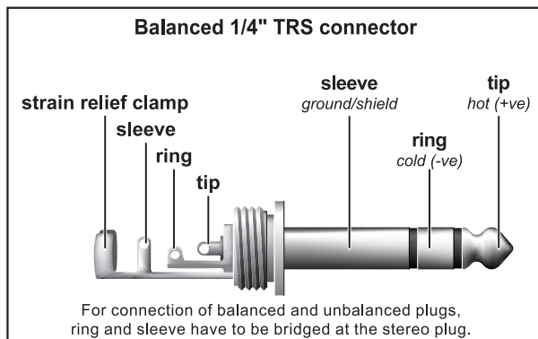
Fig. 4.2: 1/4" stereo plug
