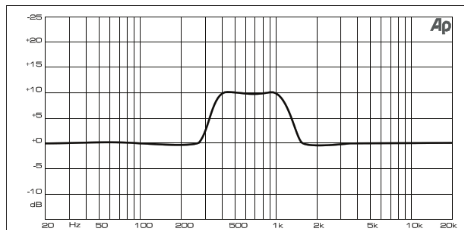
Graphic equalizer with frequency response correction.
