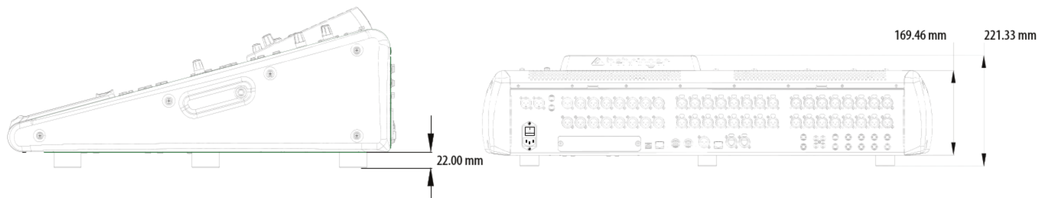
Side view
