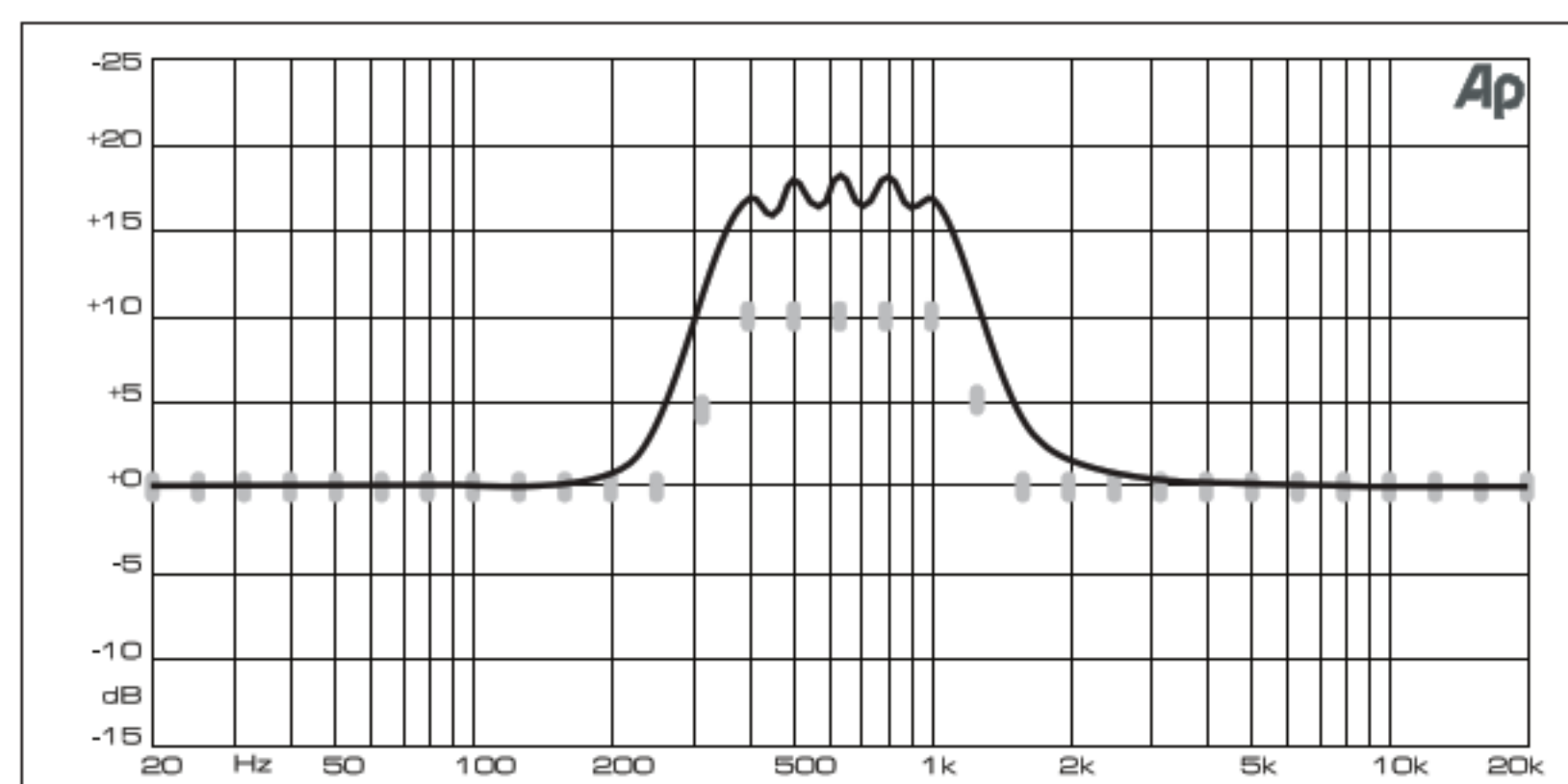
Graphic equalizer without frequency response correction.
