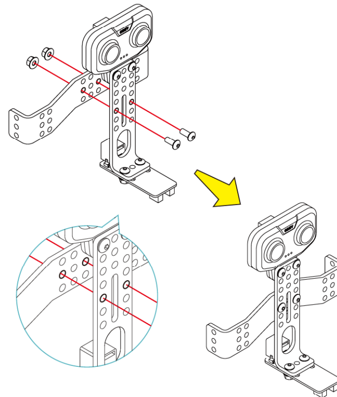
Step 6: attach the ultrasonic sensor and tracking sensor to the front bracket
