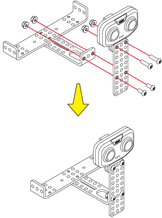
Step 5: install ultrasonic sensor
