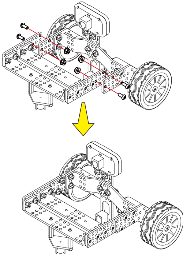
Step 10: attach the middle bracket to the front bracket
