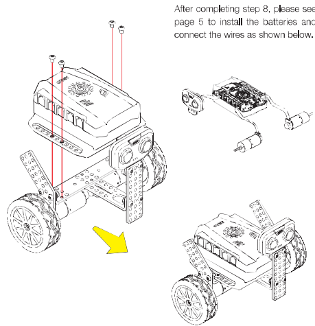
Step 8: install the main control box
