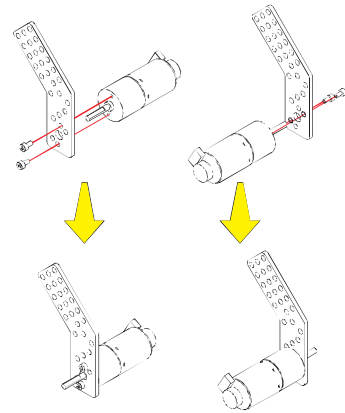
Step 1: install the right and left motor
