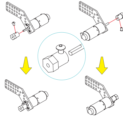
Step 2: install the right and left coupling
