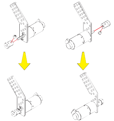
Step 2: install the right and left coupling
