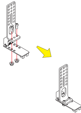
Step 9: install the tracking sensor
