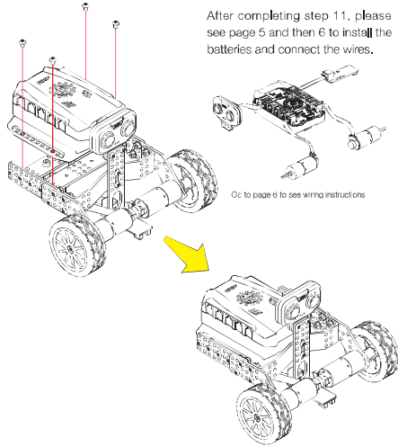
Step 12: install the main control box
