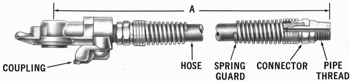
HOSE ASSEMBLIES WITH DETACHABLE FITTINGS, SPRING GUARDS AND ONE HOSE COUPLING
