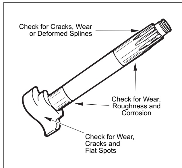
Figure 39. Camshaft Inspection
