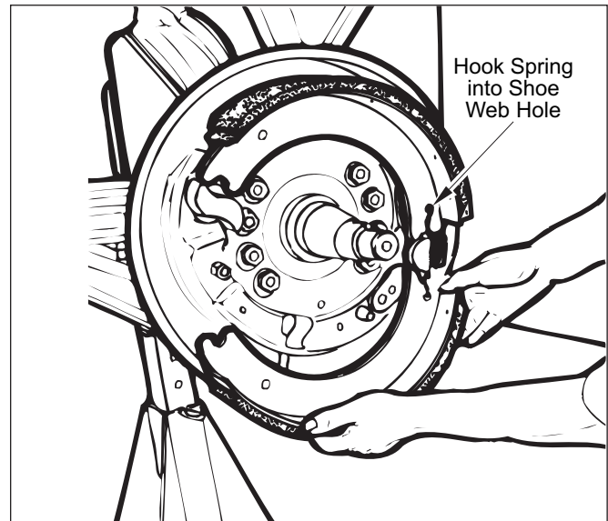
Figure 58. Shoe Retaining Spring Installation
