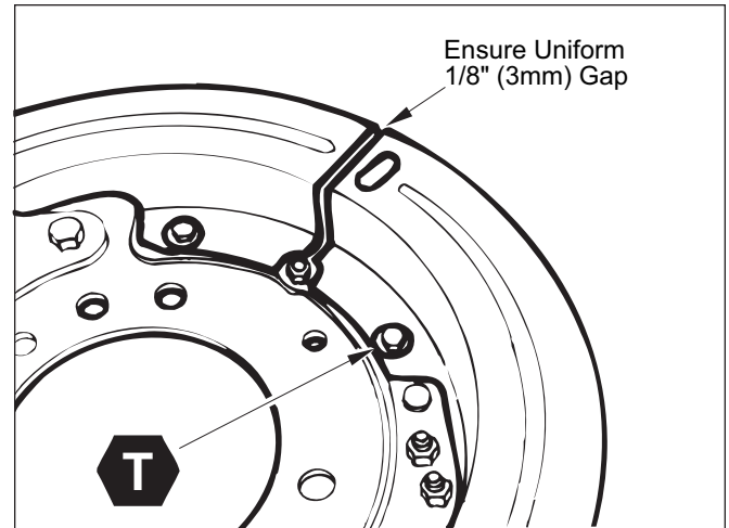
Figure 48. Dustshield Spacing
