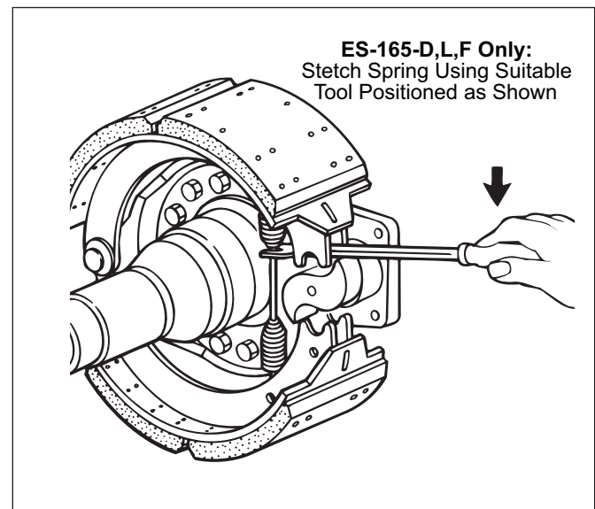
Figure 63. Shoe Return Spring Installation
