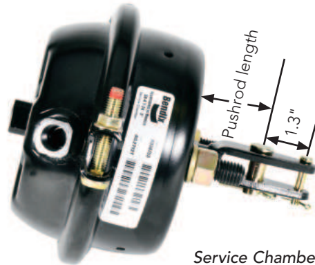
Service Chamber with welded clevis
