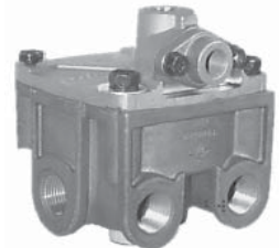
Typical Bendix® R-12DC® Relay Valve
