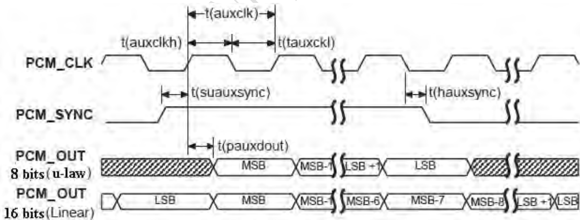
Figure 22: MODULE to EXT CODEC timing
