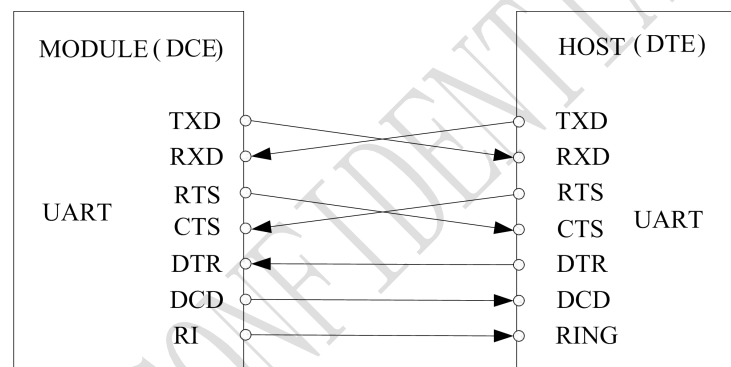
Figure 14: UART Full modem
