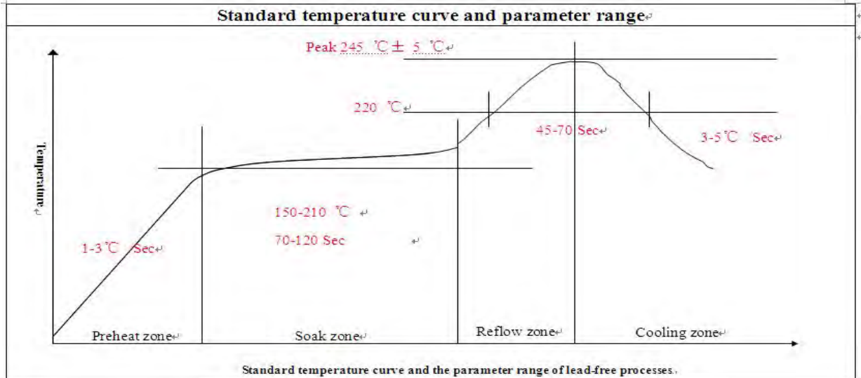
Figure 35: The ramp-soak-spike reflow profile of SIM7100C
