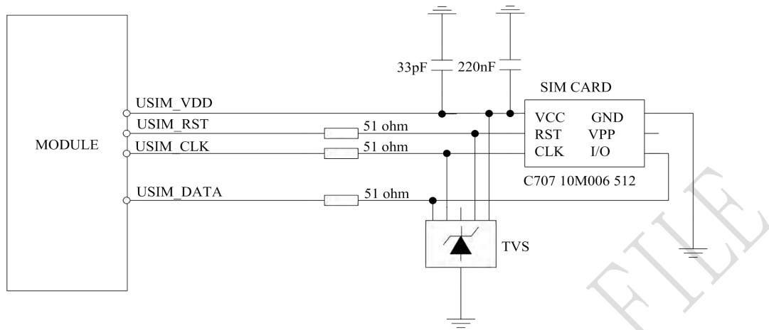
Figure 18: USIM interface reference circuit
