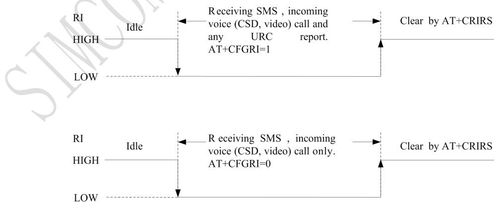
Figure 12: RI behaviour in NULL Modem
