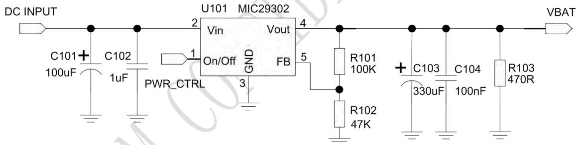
Figure 7: Reference circuit of the LDO power supply
