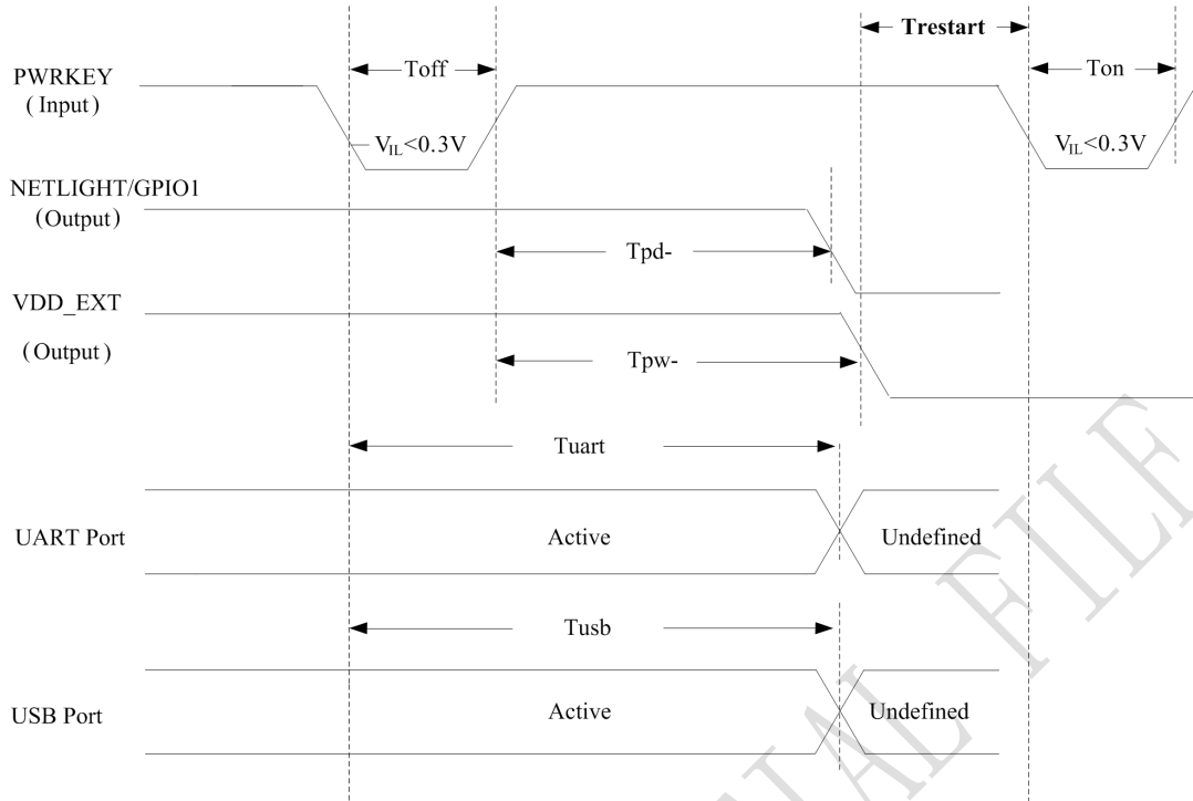
Figure 10: Power off timing sequence
