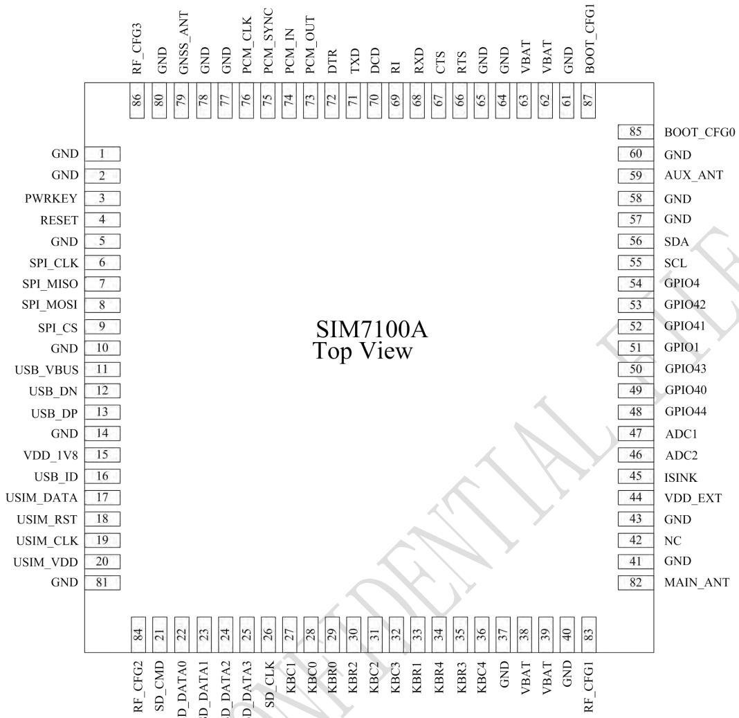
Figure 1: Pin view
