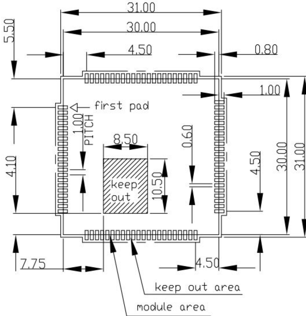
Figure 5: Footprint recommendation (Unit: mm)
