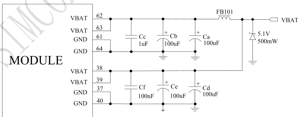
Figure 6: VBAT input application circuit
