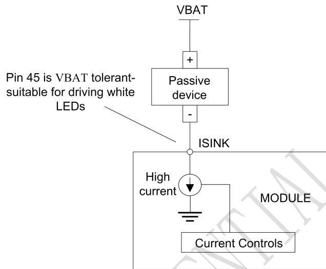
Figure 31: Current drive
