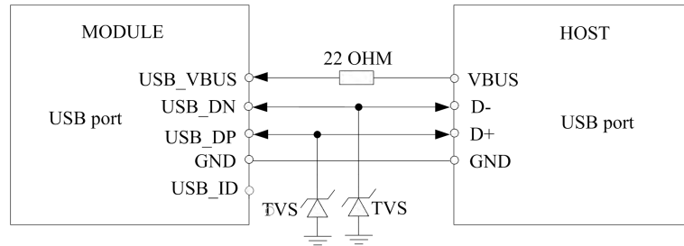
Figure 17: USB Reference Circuit with SIM7100C as USB Host Controller.
