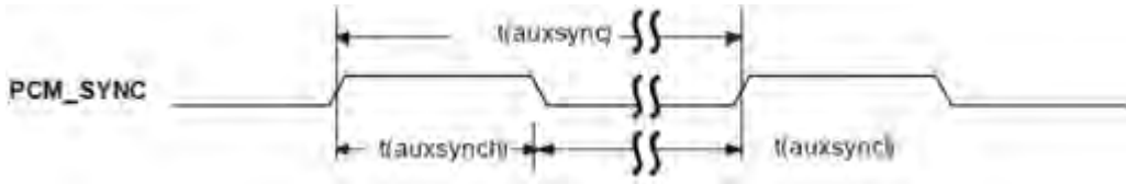
Figure 20: Synchrony timing
