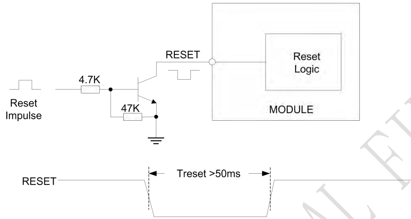
Figure 11: Reset circuit
