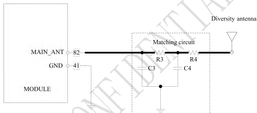
Figure 32: Antenna matching circuit (MAIN_ANT)
