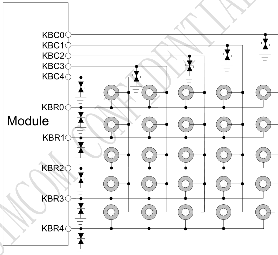
Figure 28: Reference circuit
