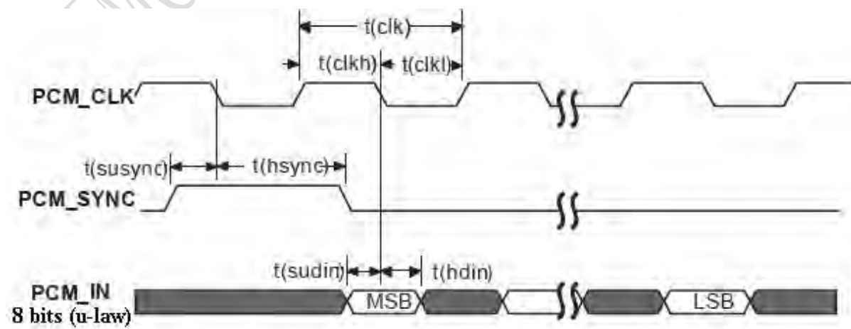
Figure 23: Synchrony timing
