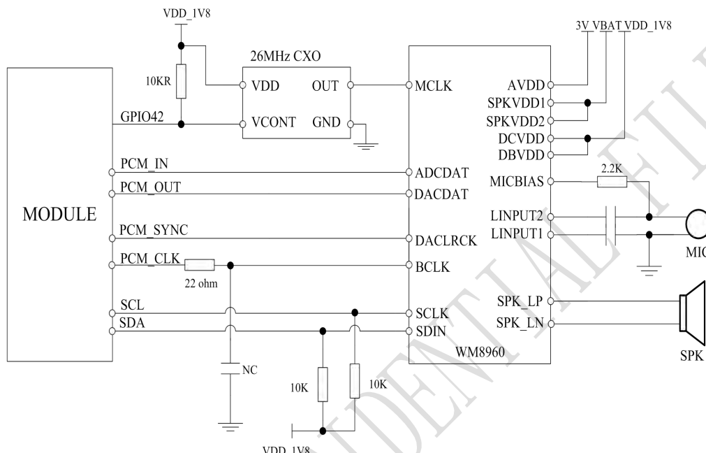
Figure 26: Reference Circuit of PCM Application with Audio Codec
