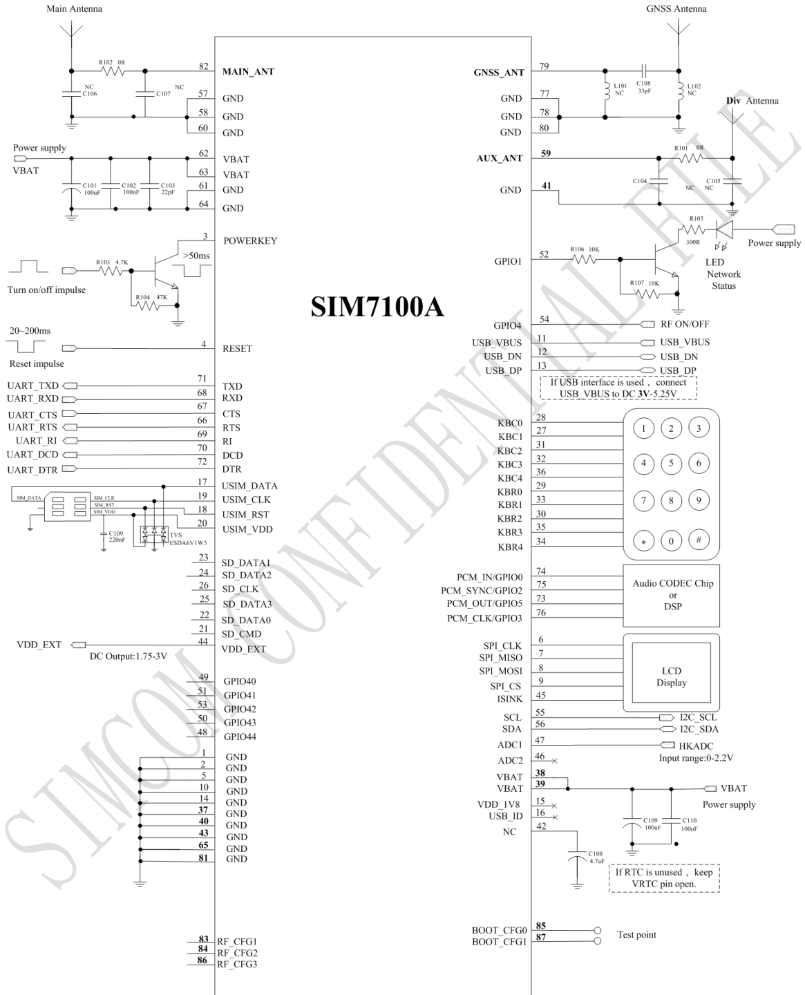
Figure 36: Reference design
