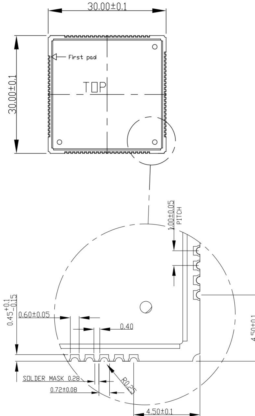
Figure 2: Top dimensions (Unit: mm)
