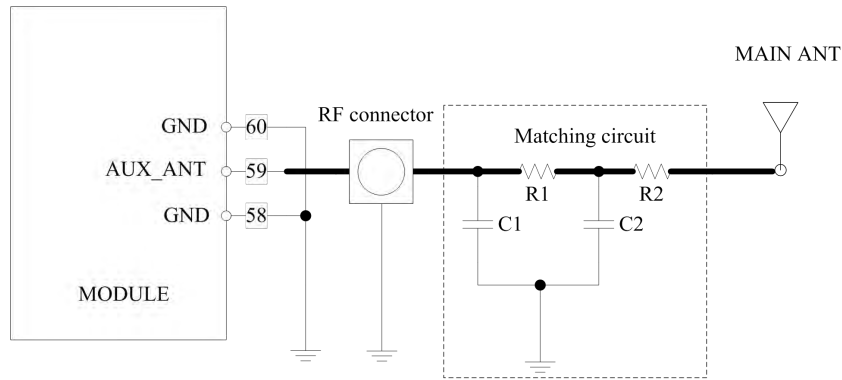
Figure 33: Antenna matching circuit (AUX_ANT)
