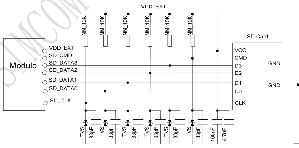
Figure 27: SD interface circuit
