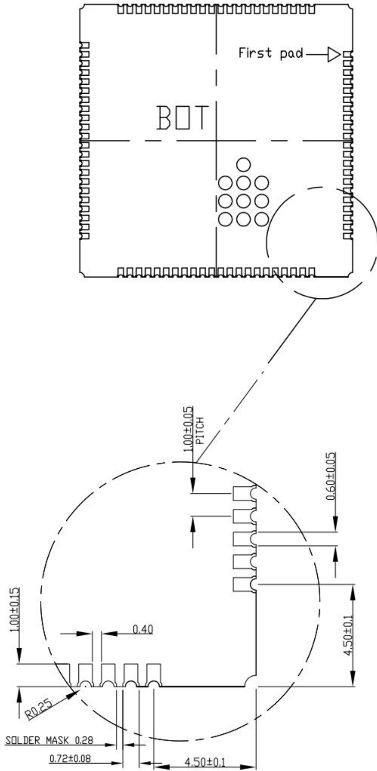
Figure 4: Bottom dimensions (Unit: mm)
