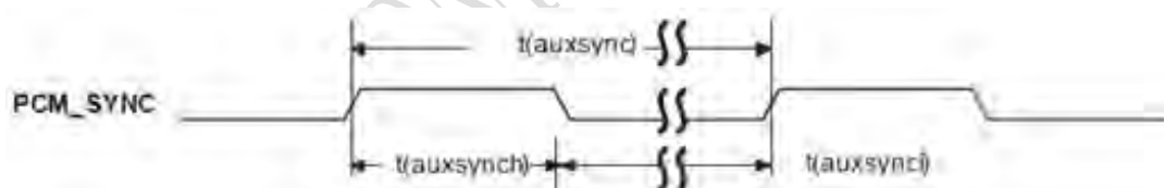
Figure 23: Synchrony timing
