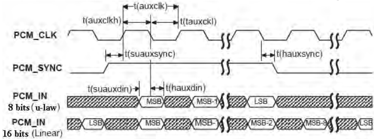
Figure 21: EXT CODEC to MODULE timing
