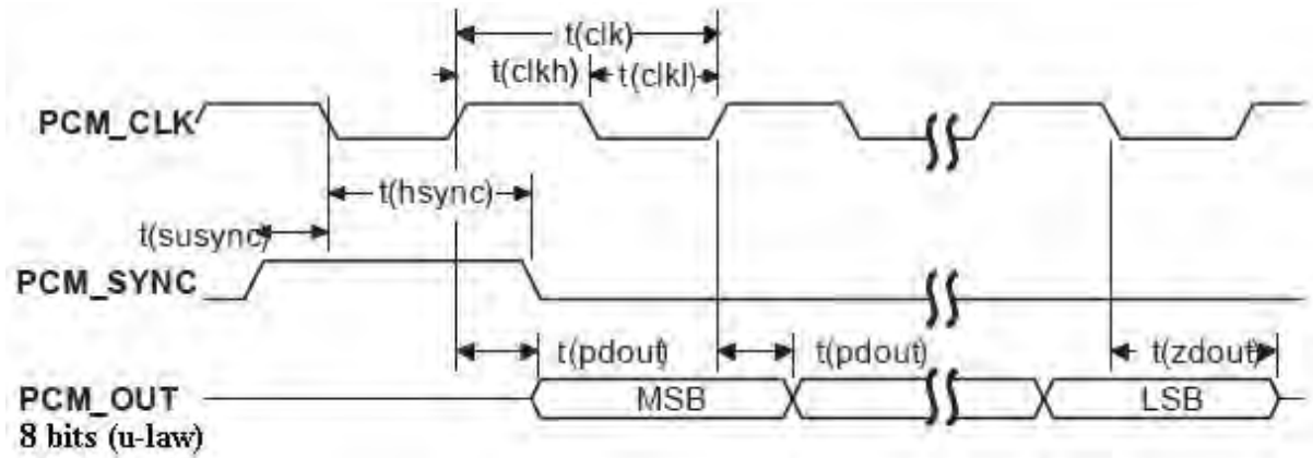
Figure 25: MODULE to EXT CODEC timing
