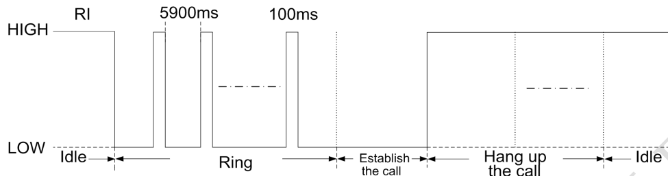
Figure 13: RI behaviour in FULL Modem
