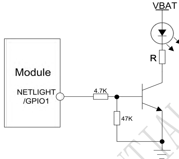
Figure 29: Application circuit
