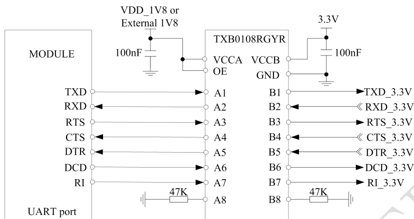
Figure 16: Reference circuit of level shift
