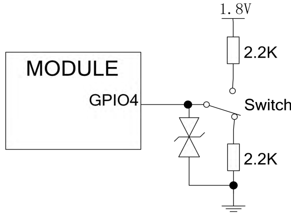
Figure 30: Flight mode switch
