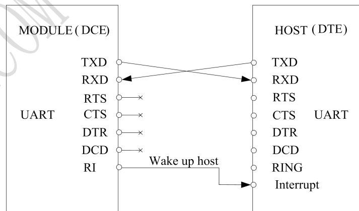
Figure 15: UART Null modem
