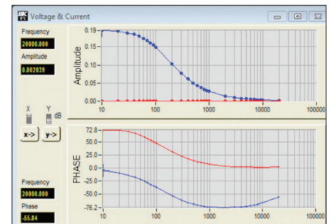
V/I plot
