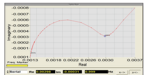
Nyquist diagram
