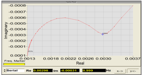
Nyquist diagram
