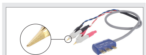
Kelvin clip test leads (TL8KC1)
