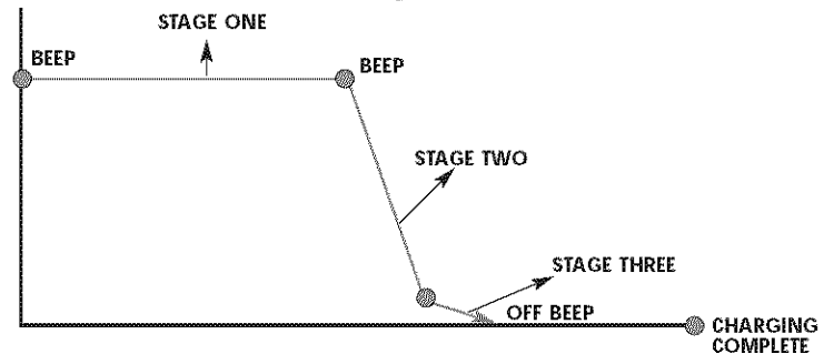
Charge Curve
