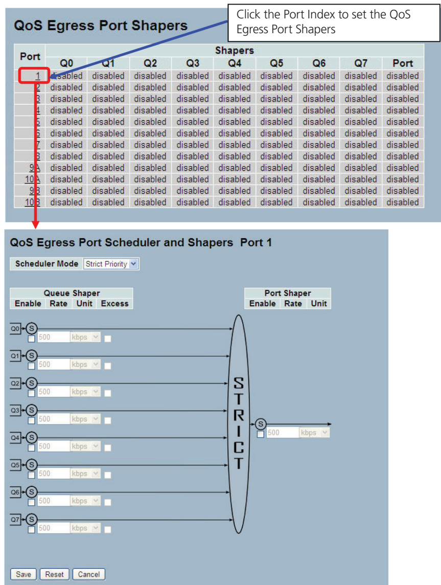
Figure 3-72. The QoS Egress Port Shapers screen, Strict Priority mode.
