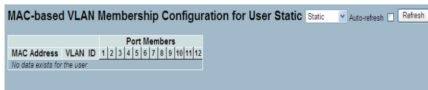
Figure 3-59. The MAC-based VLAN Membership Status for User Static screen.
