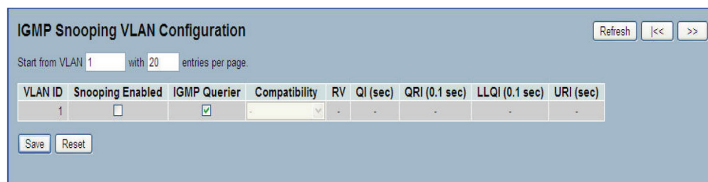
Figure 3-27. The IGMP Snooping VLAN Configuration screen.
