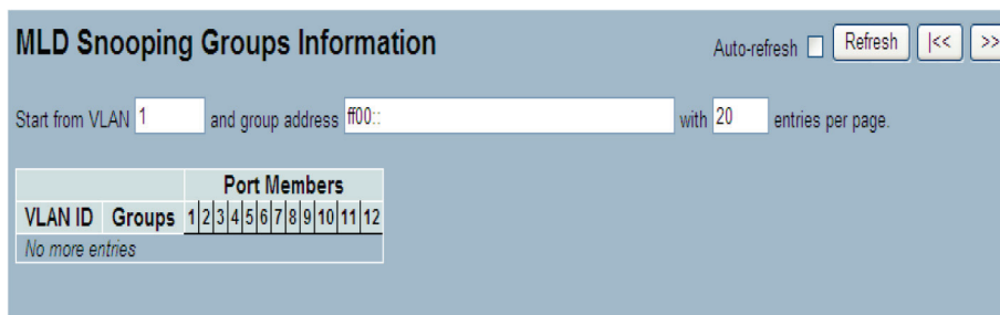
Figure 3-37. The MLD Snooping Groups Information screen.
