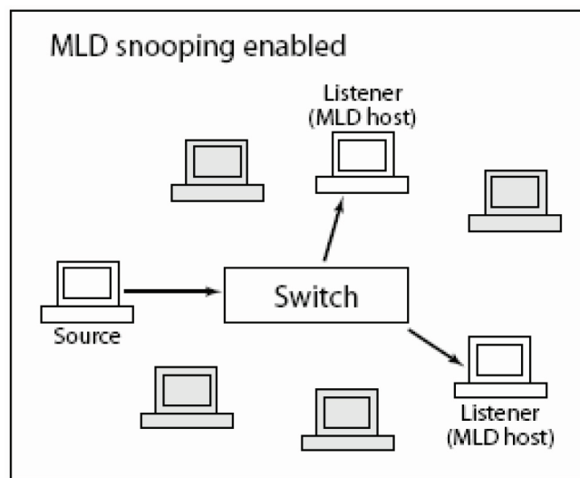
Figure 3-32. MLD Snooping Enabled screen.
