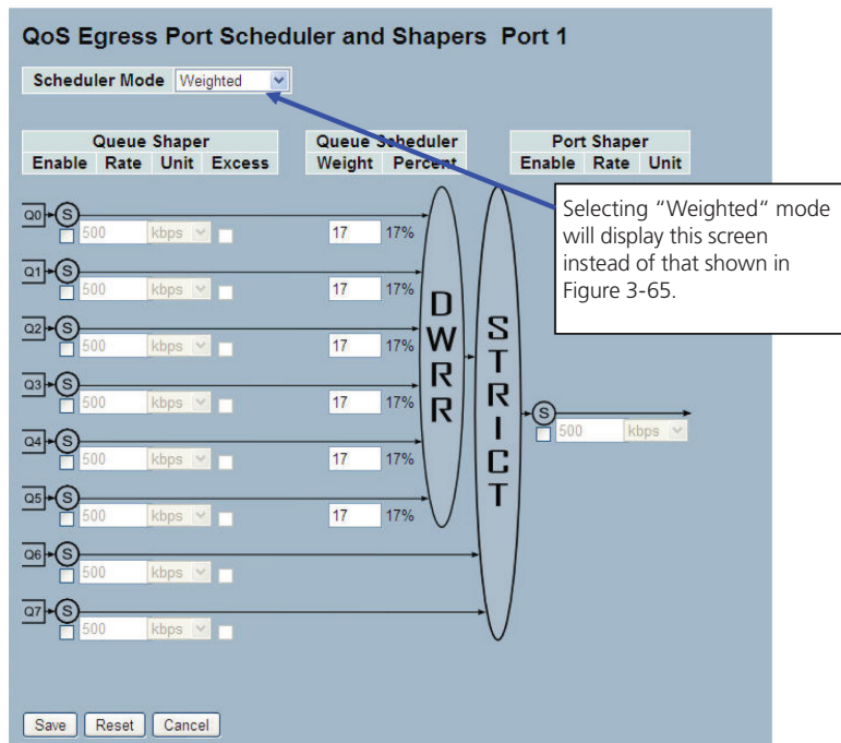
Figure 3-71. The QoS Egress Port Scheduler front screen in Weighted mode.
