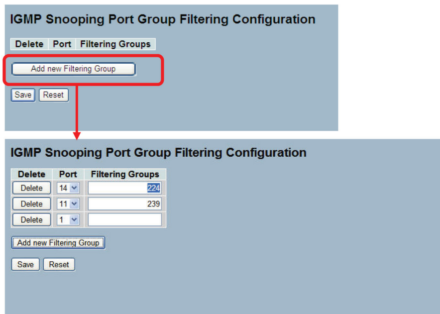
Figure 3-28 The IGMP Snooping Port Group Filtering Configuration screen.
