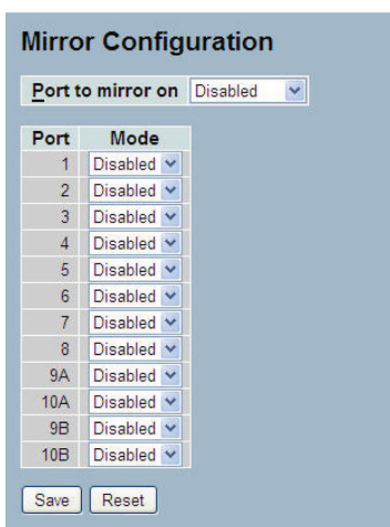
Figure 3-91. The Mirror Configuration screen.
