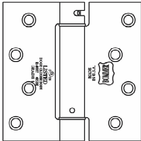
LB4362-400 4" X 4" Square Castlegate Door
