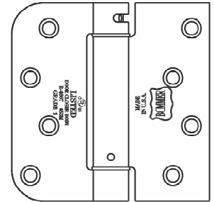
LB4361-400 4" X 4" 5/8" Radius Leaf / Square Leaf Castlegate Door
