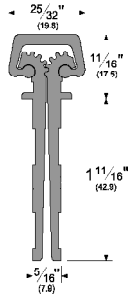
Full Mortise Short Leaf Flush
