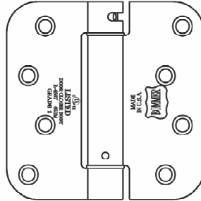
LB4322-400 4" X 4" 5/8" Radius Perma-Door
