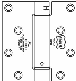
LB4350-400 4" X 3 3/4" Square Acorn Door
