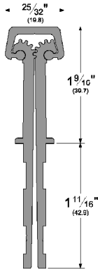
Wide Throw Full Mortise
