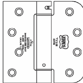
LB4376-400 4" X 4" Square Leaf / 5/8" Radius Leaf Johnson Integrity
