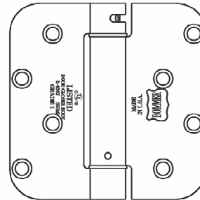
LB4360-400 4" X 4" 5/8" Radius Acorn Door
