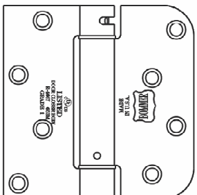
LB4381-400 4" X 4" Square Leaf / 5/8" Radius Leaf Stanley Door System
