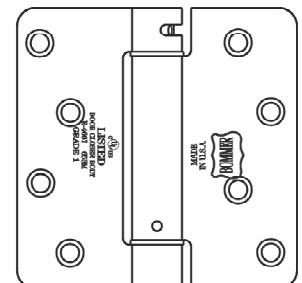
LB4384-400 4" X 4" 1/4" Radius Taylor Door
