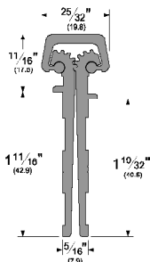
Full Mortise Short Leaf Inset
