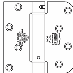
LB4377-400 4" X 4" Square Leaf / 5/8" Radius Leaf Reeb
