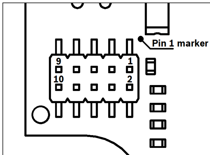
Figure 4 Debugger connector
