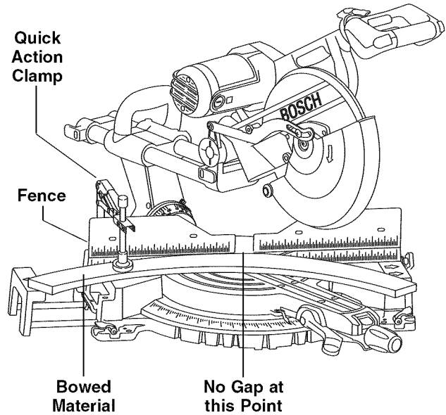
Figure 37. Bowed Material
