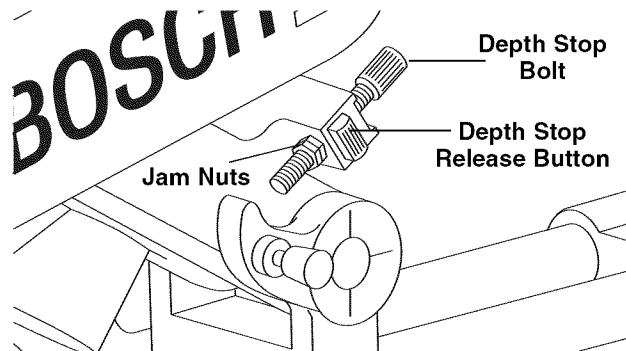
Figure 33. Cutting Grooves
