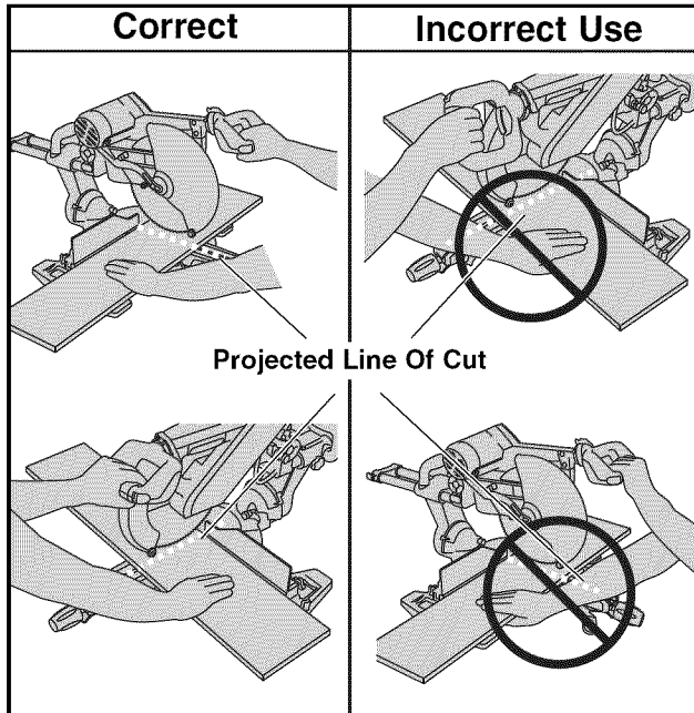
Figure 17. Hand Positions
