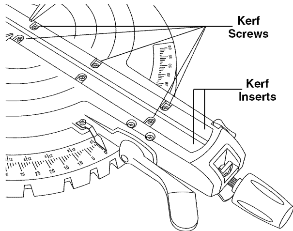
Figure 12. Kerf Insert
