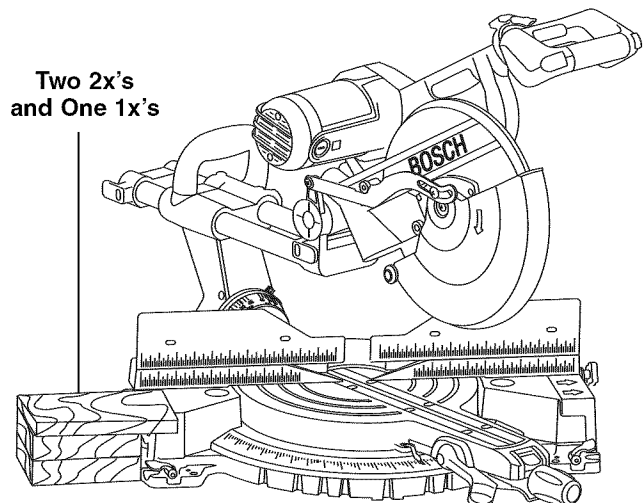
Figure 21. Block Support
