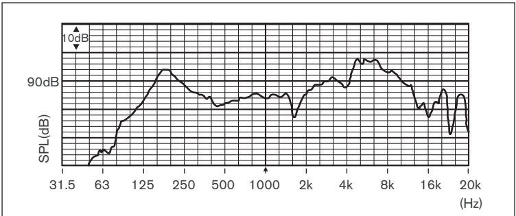
Frequency response
