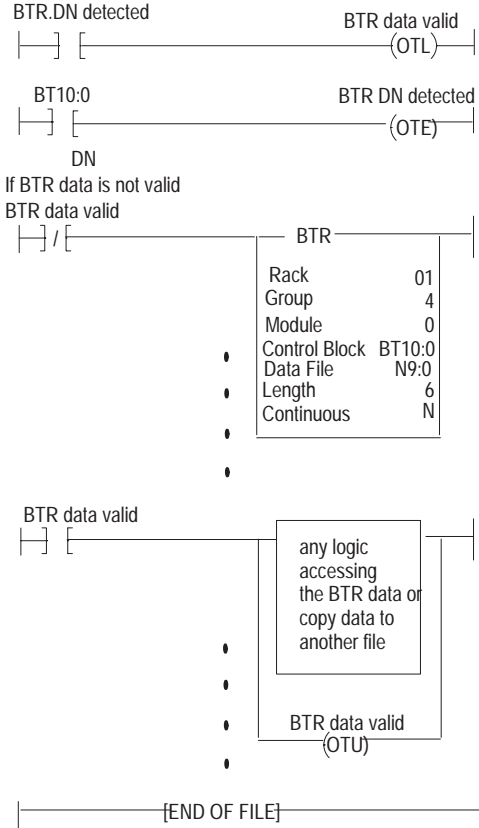
After the BTR done bit is set, the valid data in the BT data buffer is copied to the BTR data table file during housekeeping.
