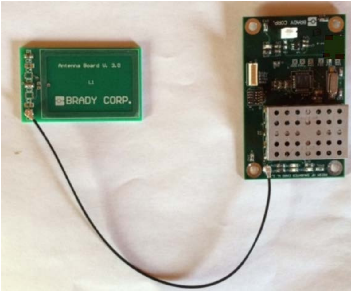
Figure 2. photo of the Brady BDC2000 RFID Assembly
