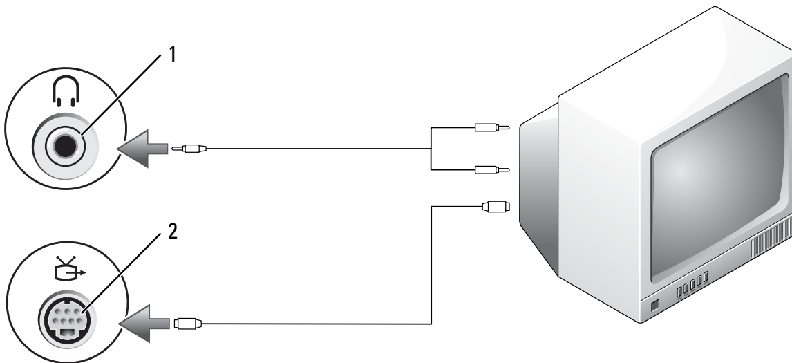
1 audio connector 2 S-video TV-out connector
