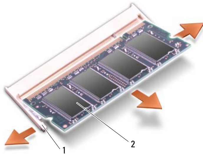
1 securing clips (2) 2 memory module
