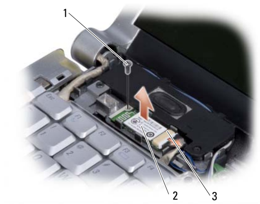
1 screw 2 card 3 cable connector
