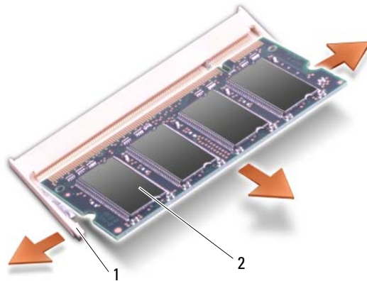
1 securing clips (2) 2 memory module
