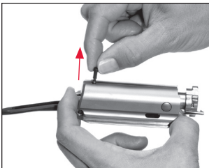
Remove the firing pin retaining pin.
