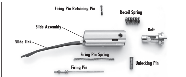
The slide assembly shown disassembled for cleaning.
