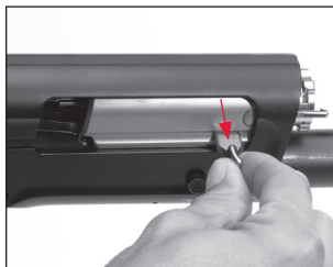
Pull outward to remove the operating handle.
