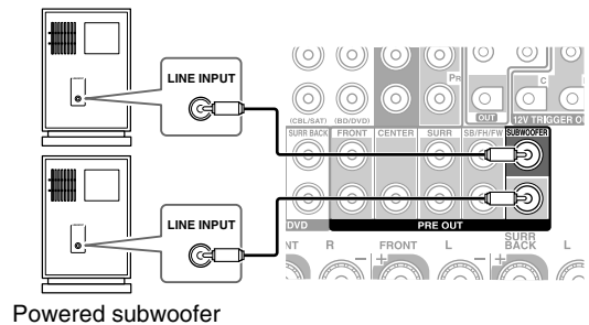
Powered subwoofer
