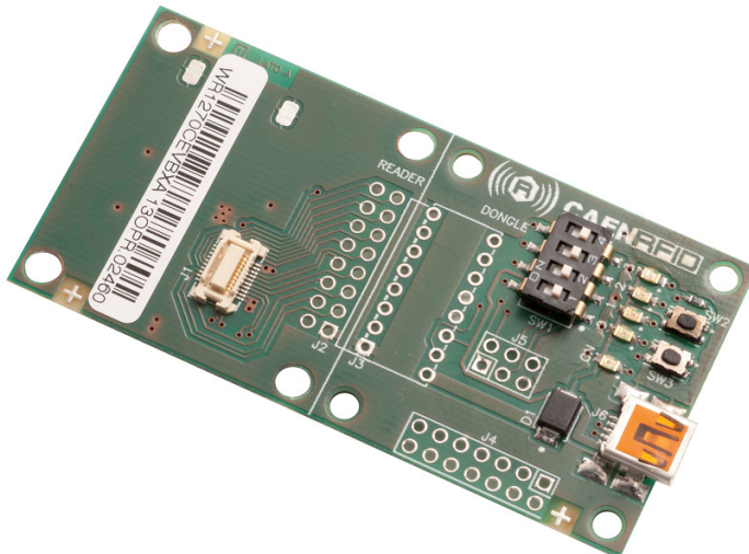
Fig. 1.2: Quark Up R1270CEVB - Quark-Up Reader Evaluation Board
