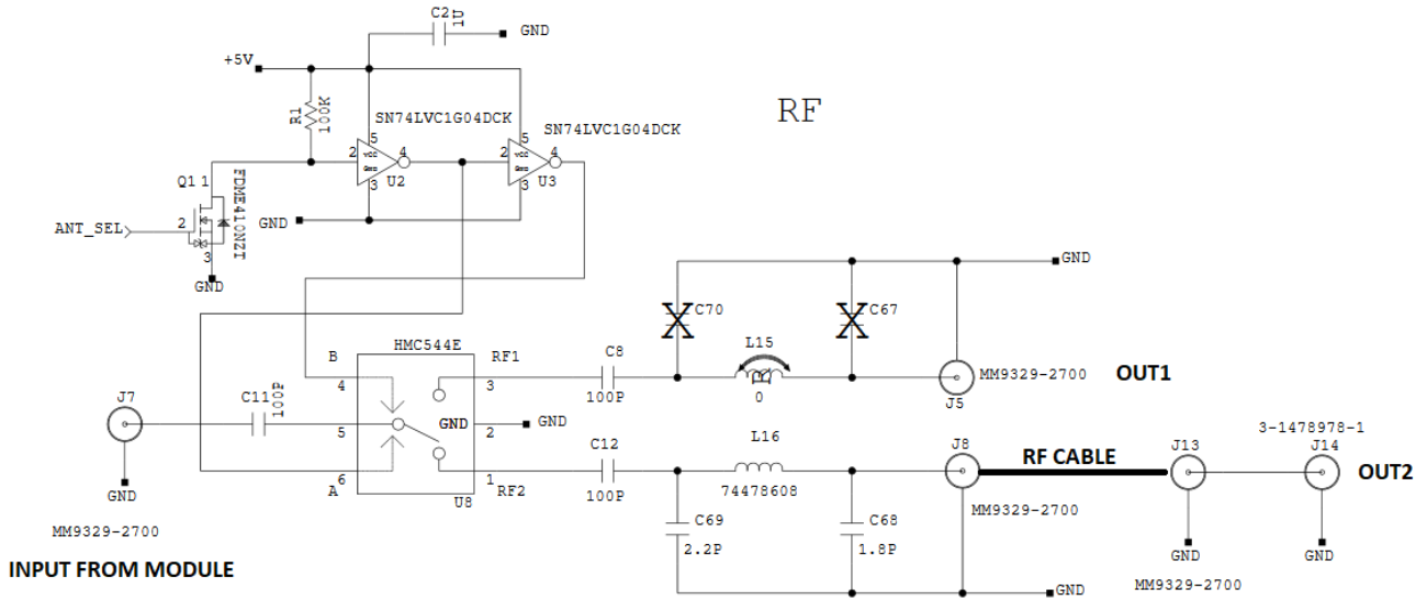
Fig. 7: Dual multiplexed antenna application note
