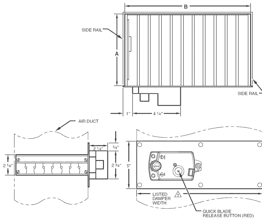
Fig. 2 – Bottom-Mount Damper Configuration
