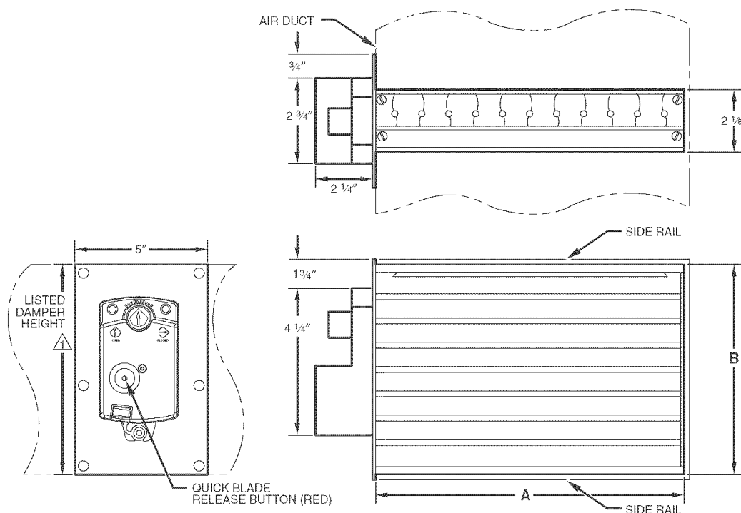
Fig. 1 – Side-Mount Damper Configuration
