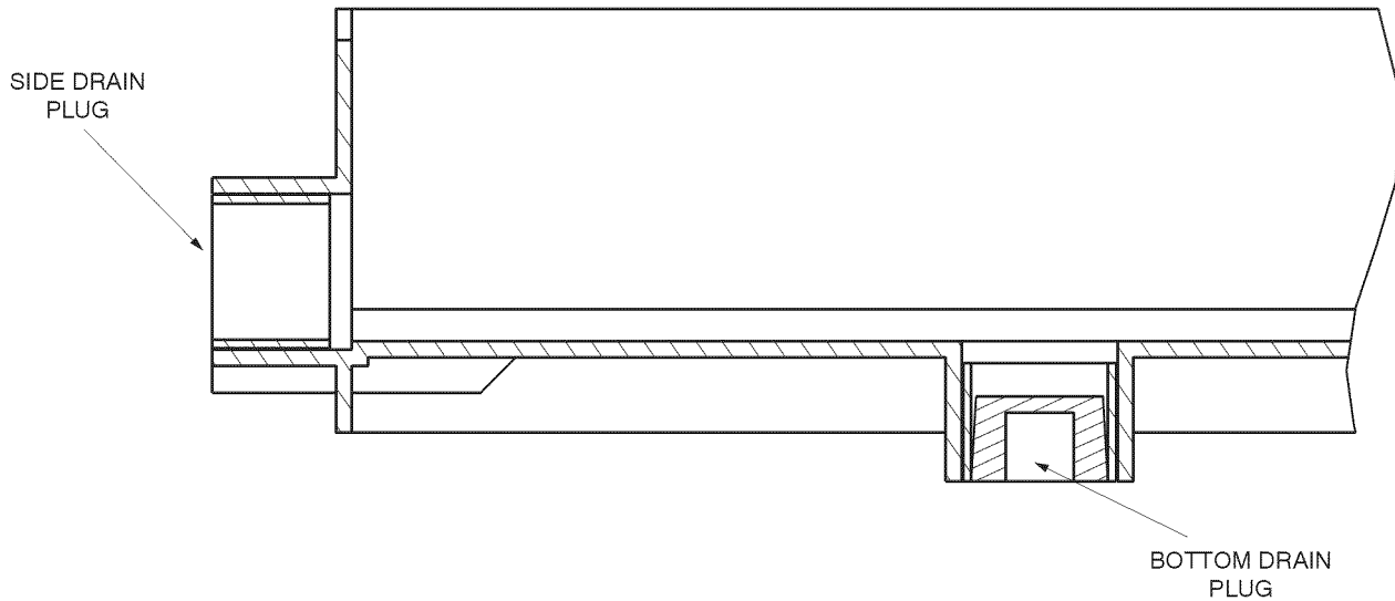
Fig. 5 - Condensate Drain Piping Details
