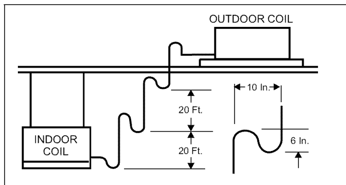
FIGURE 2: Oil Trap
