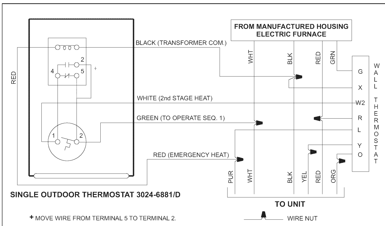
FIGURE 12 - Wiring Connections for BRHQ, DRHQ Series (Revision A, B, or C)
