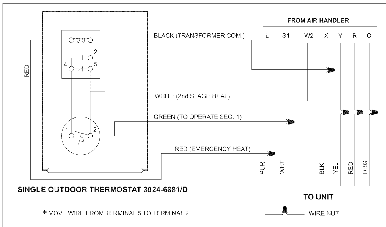
FIGURE 11 - Wiring Connections for BRHS, DRHS Series (Revision A, B, or C)
