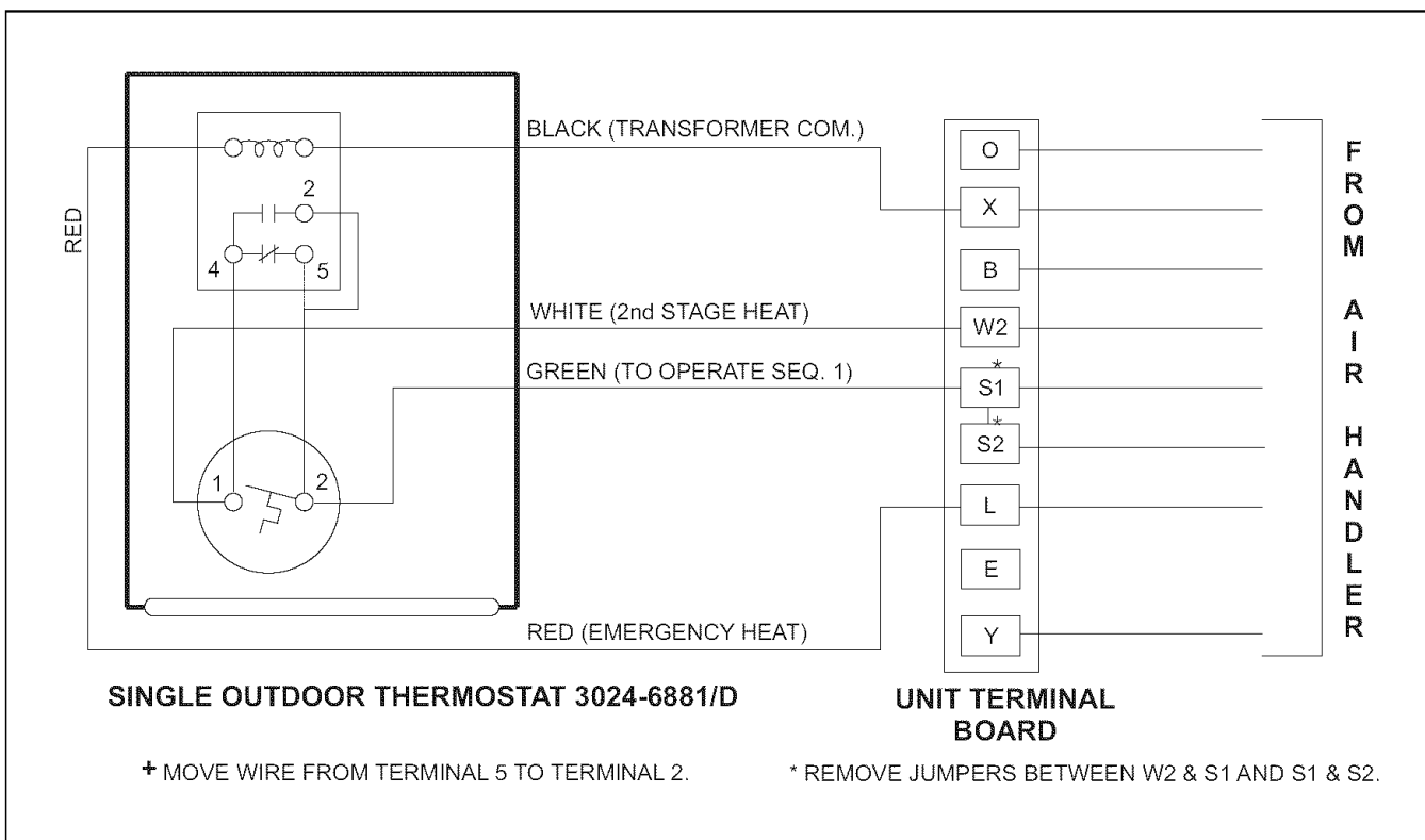
FIGURE 9 - Wiring Connections for FRHS Series (Revision A, B, or C)
