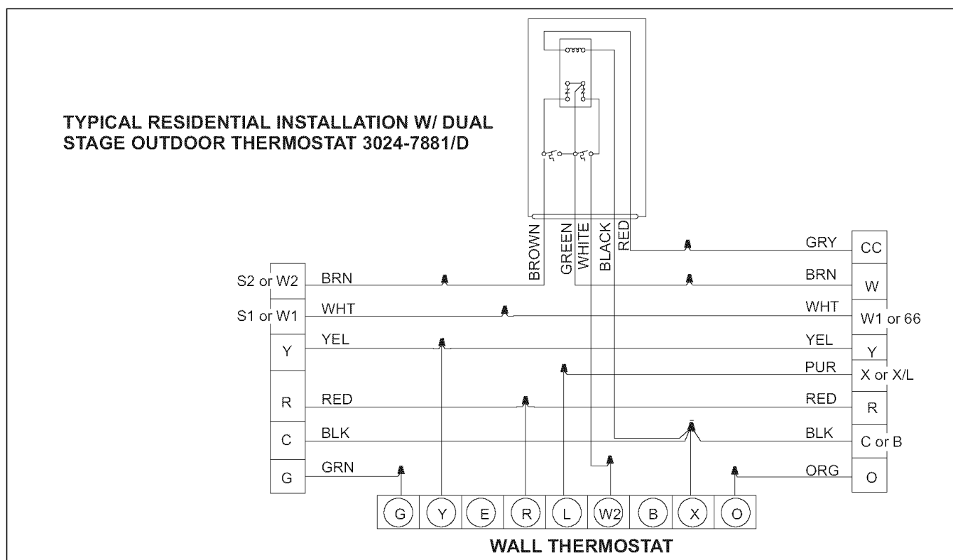
FIGURE 2 - Wiring Connections for BRHS, DRHS, FRHS, BH(Q)< DH(Q)< or FH with Revision Code of "D" or Higher
