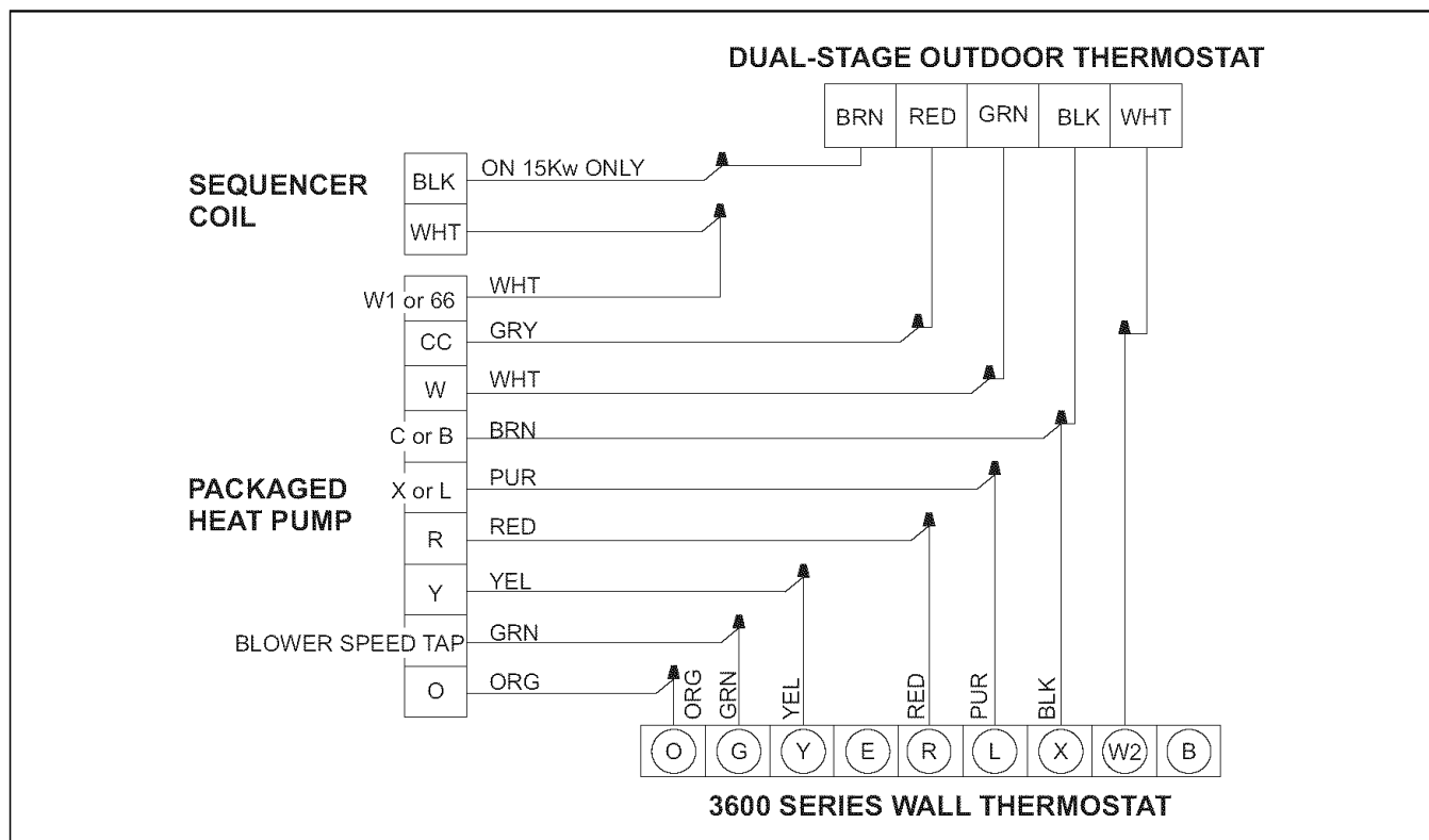
FIGURE 7 - Wiring Connections for JP/PHP Packaged 13 SEER Heat Pump
