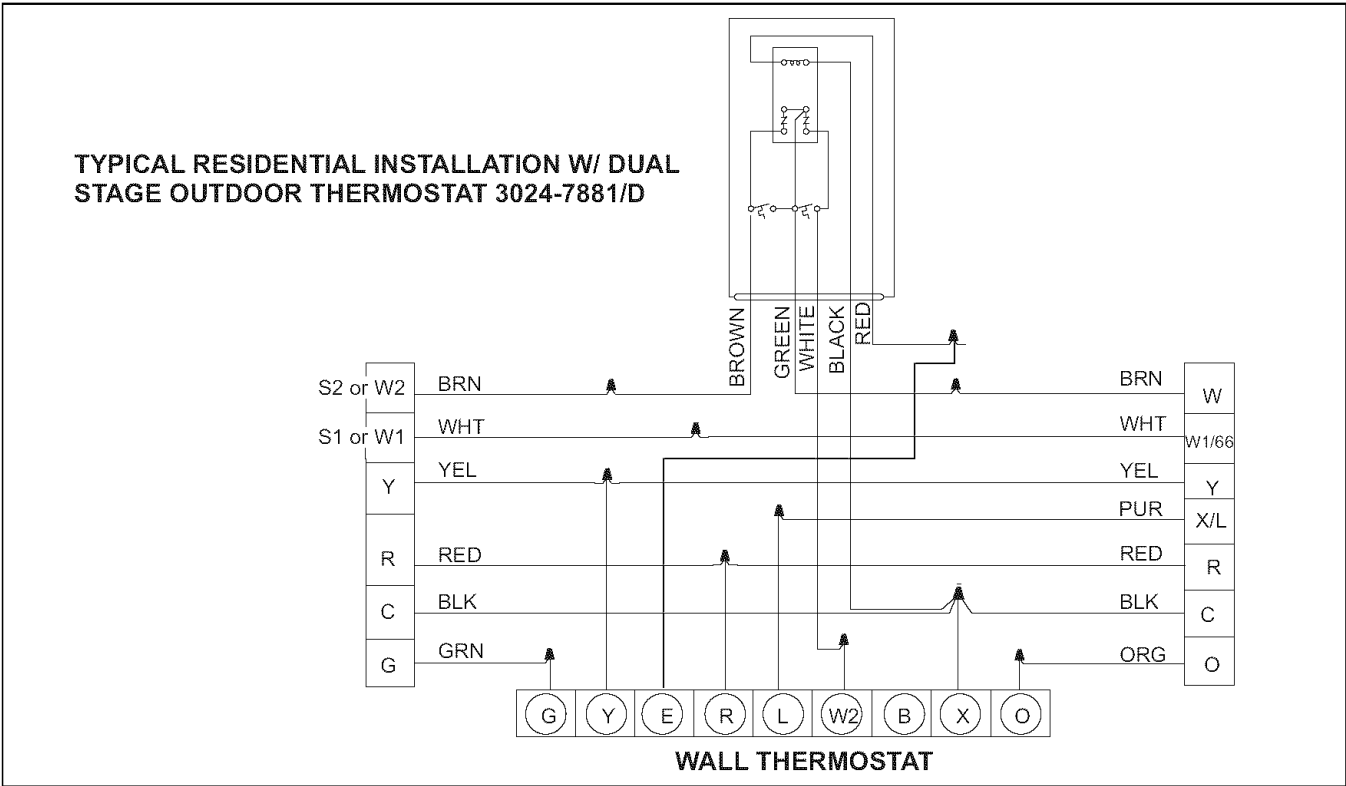
FIGURE 14 - Wiring Connections for ERHS and ERHQ using Demand - Defrost Board
