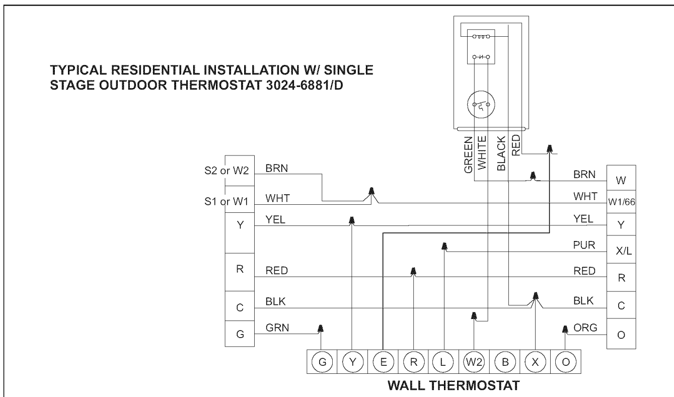
FIGURE 13 - Wiring Connections for ERHS and ERHQ using Demand - Defrost Board
