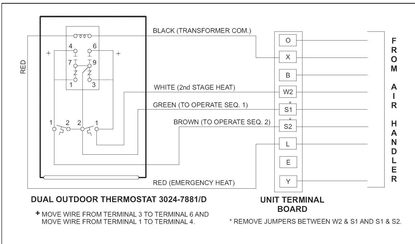
FIGURE 8 - Wiring Connections for FRHS Series (Revision A, B, or C)
