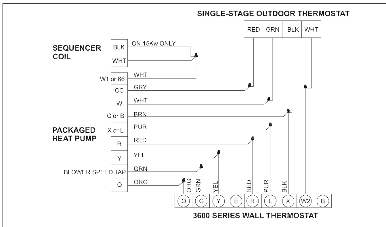
FIGURE 6 - Wiring Connections for JP/PHP Packaged 13 SEER Heat Pump
