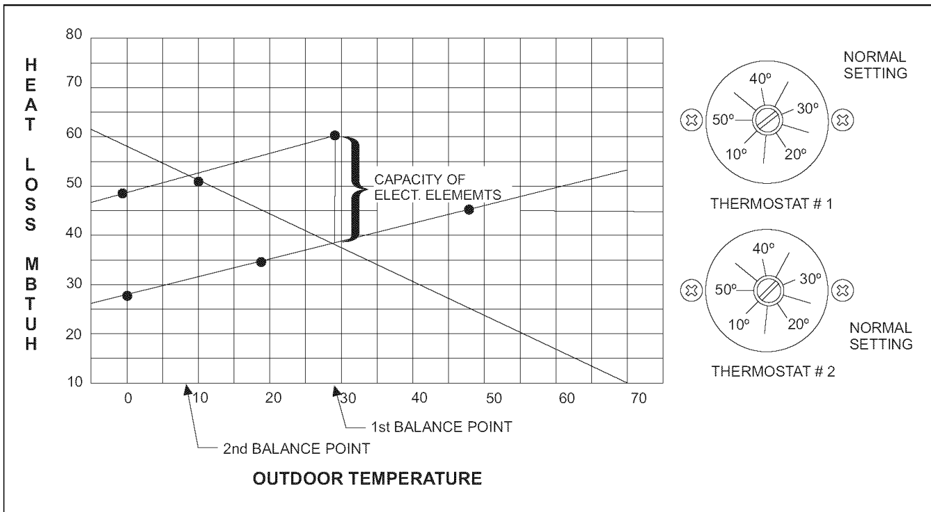
FIGURE 17 - Balance Point Determination Chart
