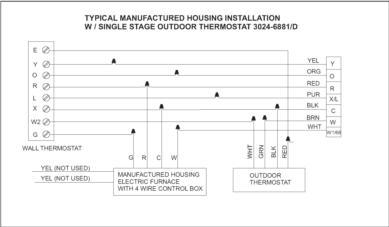
FIGURE 15 - Wiring Connections for ERHS and ERHQ using Demand - Defrost Board
