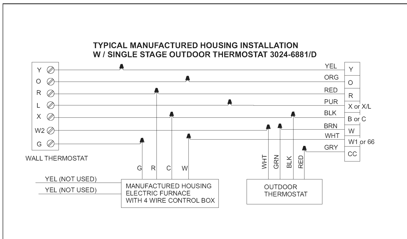
FIGURE 3 - Wiring Connections for BRHQ, DRHQ with Revision Code of "D" or Higher
