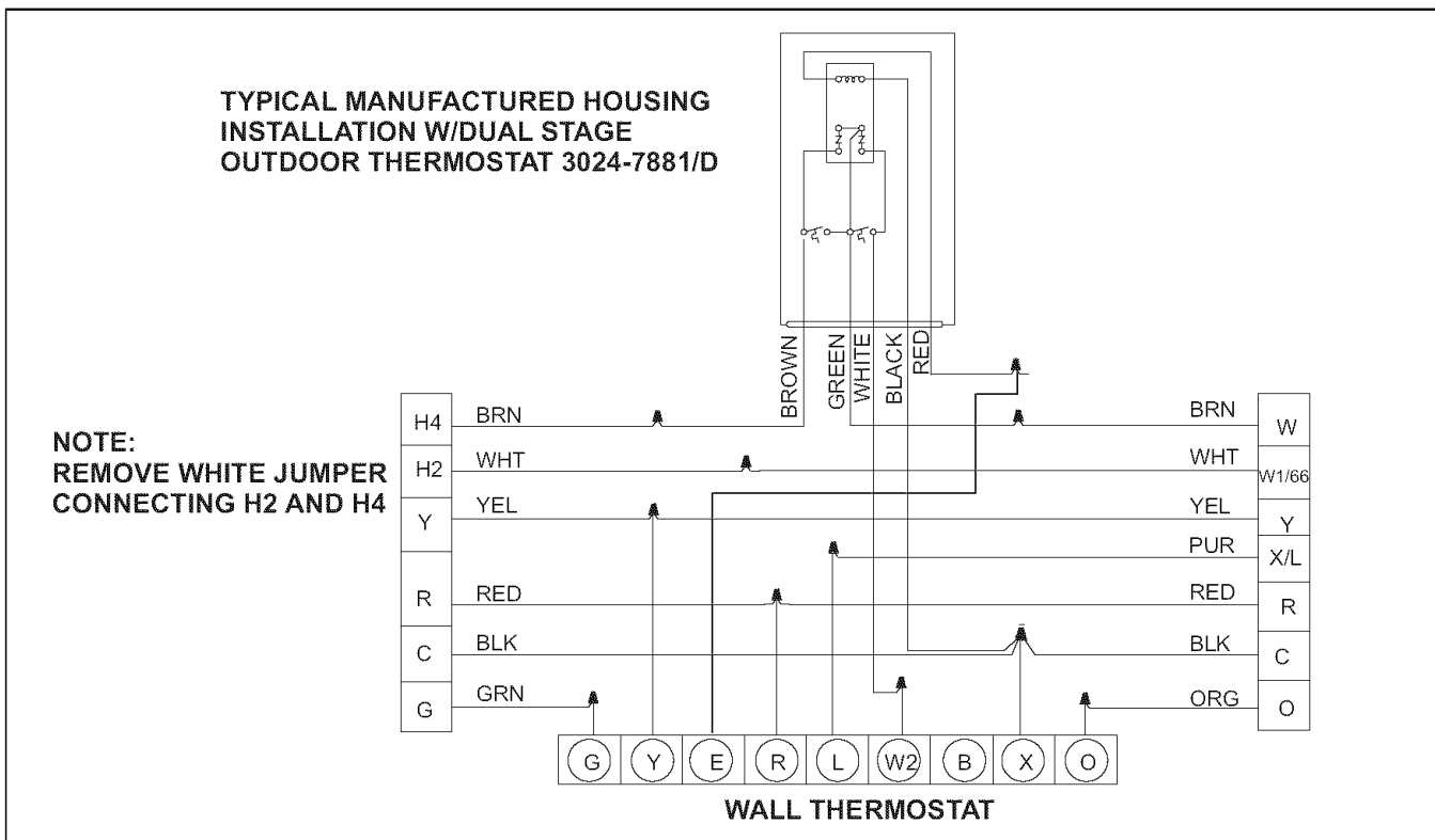
FIGURE 16 - Wiring Connections for ERHS and ERHQ using Demand - Defrost Board
