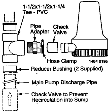
Figure 2B – Installation Diagram
