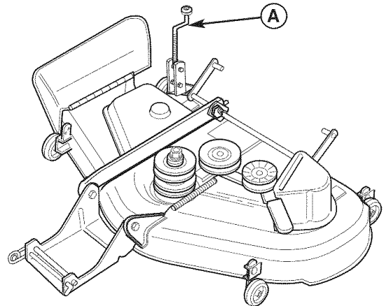
Figure 35. Cutting Height Adjustment A. Cutting Height Adjustment Crank
