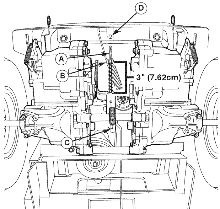
Figure 36. Brake Adjustment
