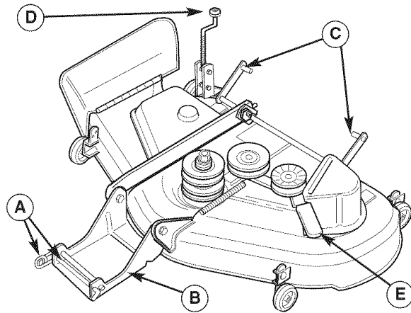
Figure 10. Mower Components
