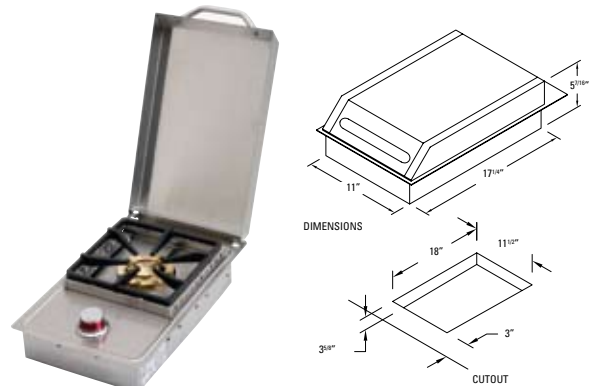
Standard Single Flat Side Burner Part Number: BBQ08852P
