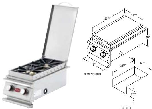
Deluxe Double Side Burner Part Number: BBQ08899P
