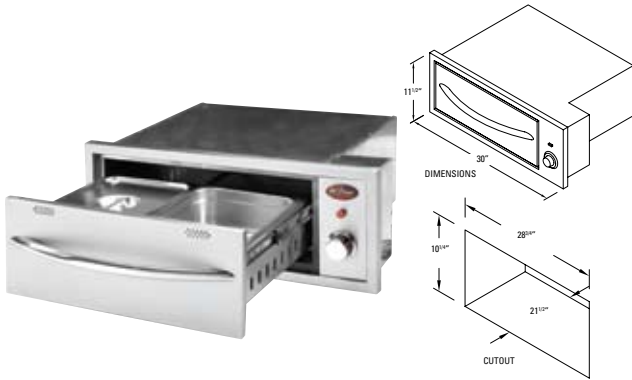
30" Warmer Drawer Part Number: BBQ07889P
