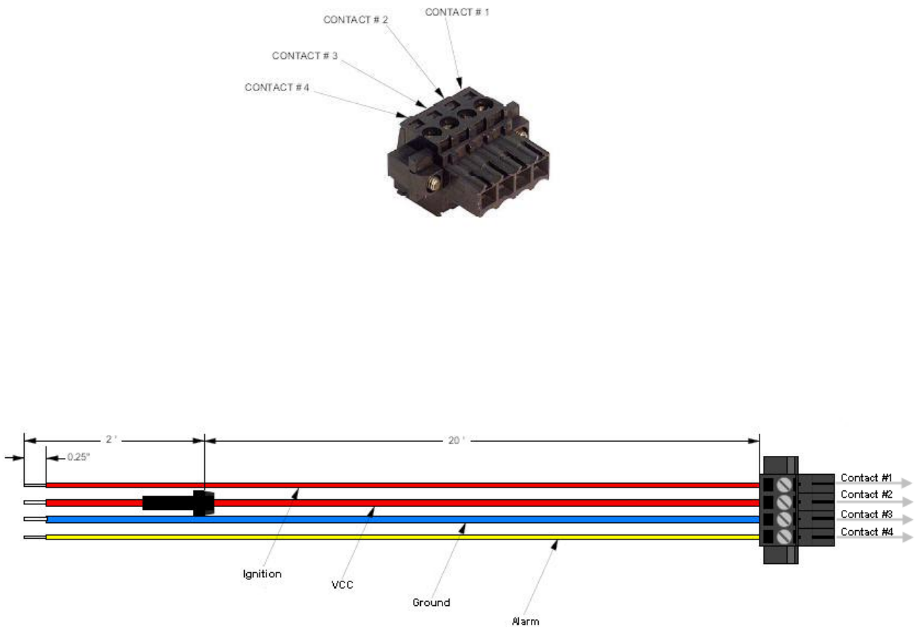
Figure 2 – Sentry 4G Power Cable Connections
