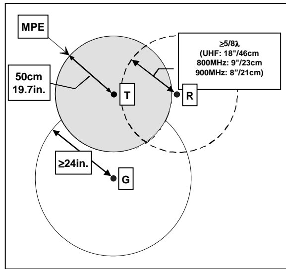
Figure 4 - Antenna spacing
