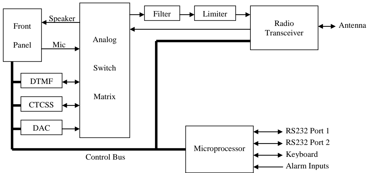
Peoplefinder II Block Diagram
