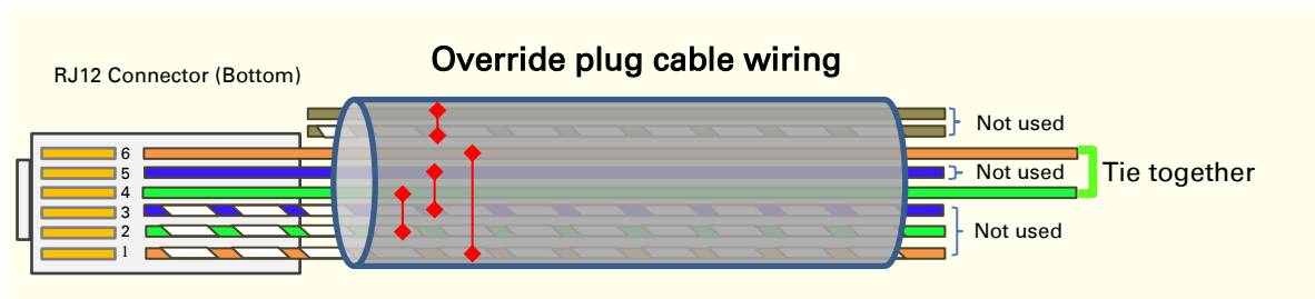
Figure 47 RJ-11 pinout for the default plug
