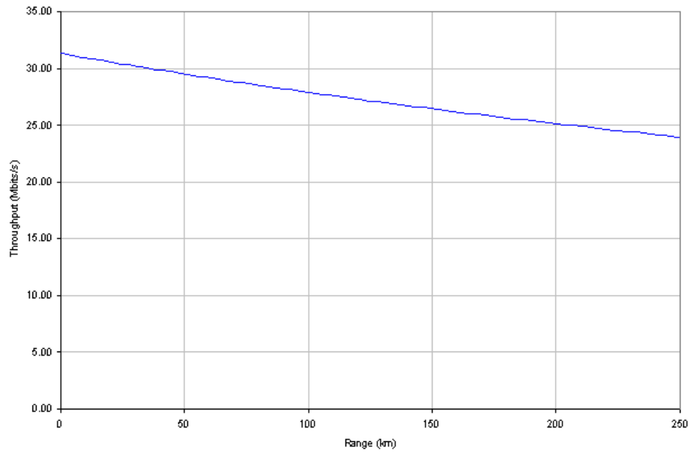
Figure 118 - QPSK 0.75 Dual Payload
