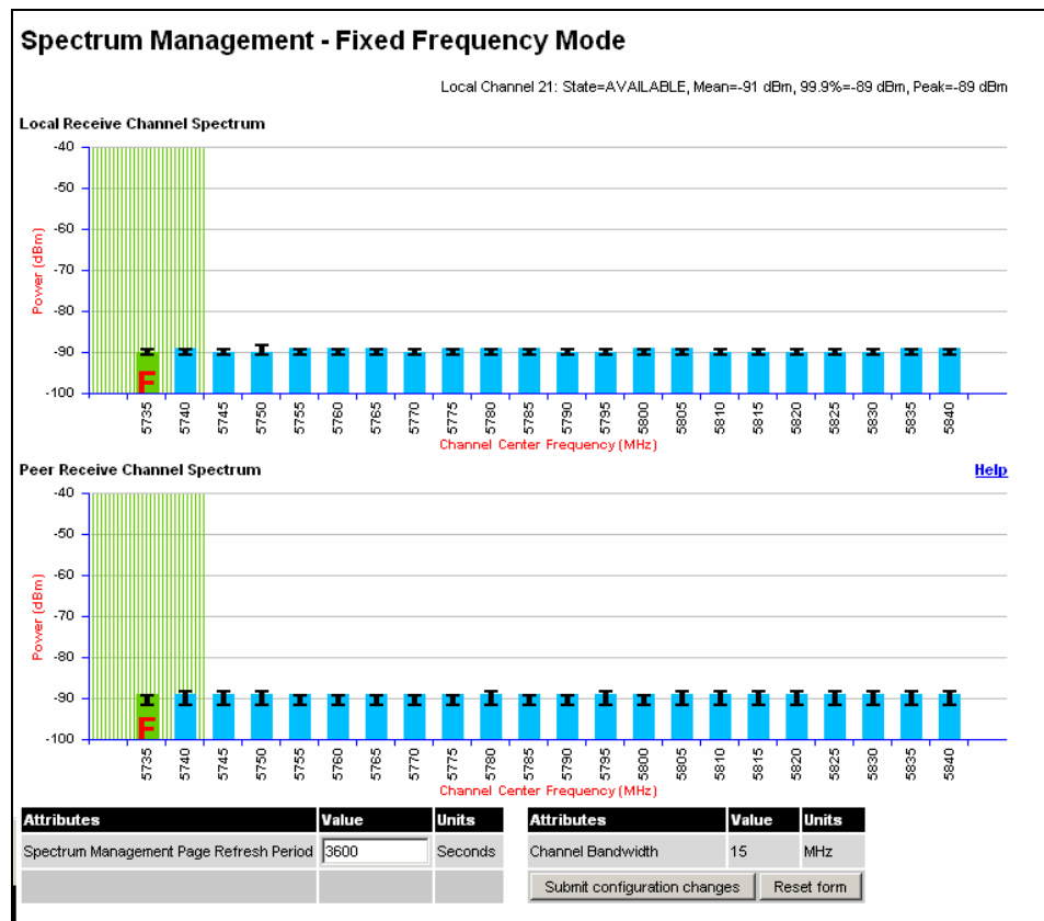
Figure 62 - Spectrum Management Fixed Frequency Screen
