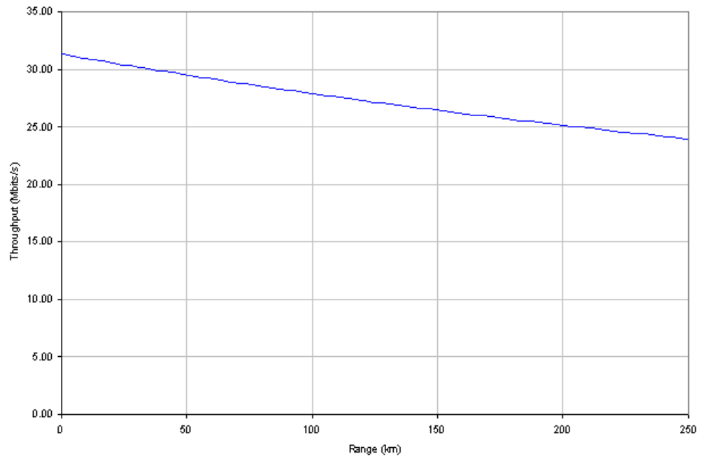
Figure 114 - 16 QAM 0.75 Single Payload
