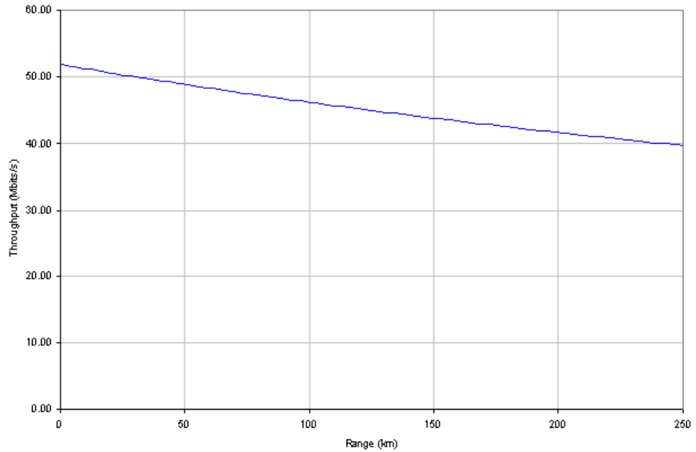
Figure 116 - 64 QAM 0.83 Single Payload
