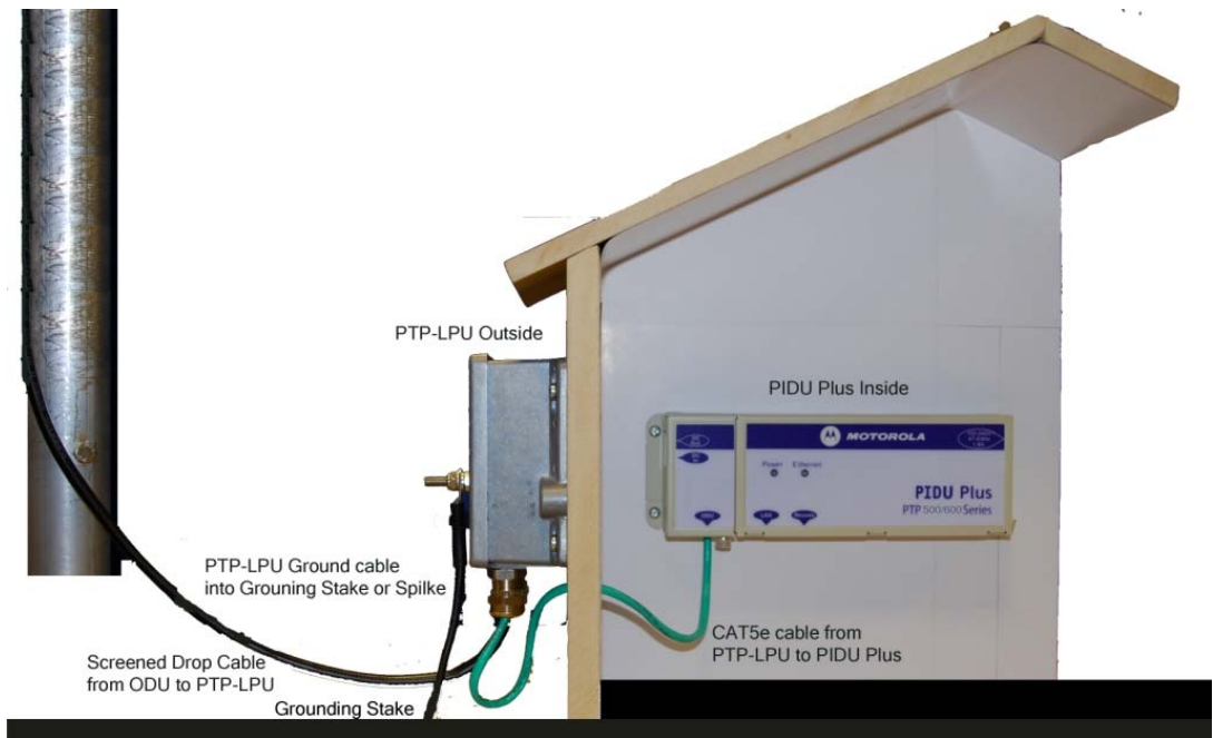
Figure 95 - PTP LPU Installation Example for PTP 500 Series (Not to Scale)
