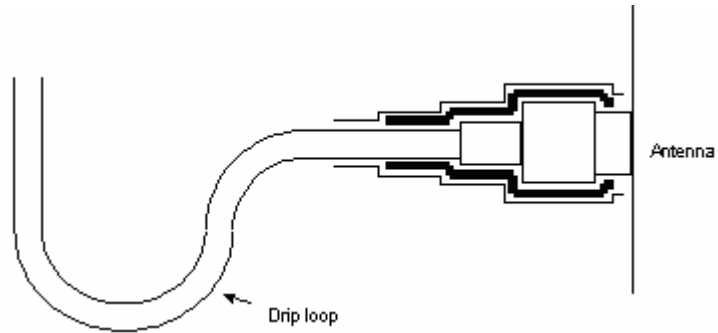
Figure 105 - Forming a Drip Loop
