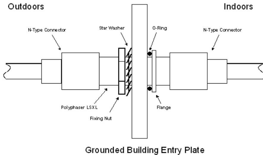
Figure 109 - Polyphaser Assembly
