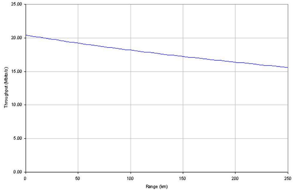
Figure 113 - 16 QAM 0.50 Single Payload
