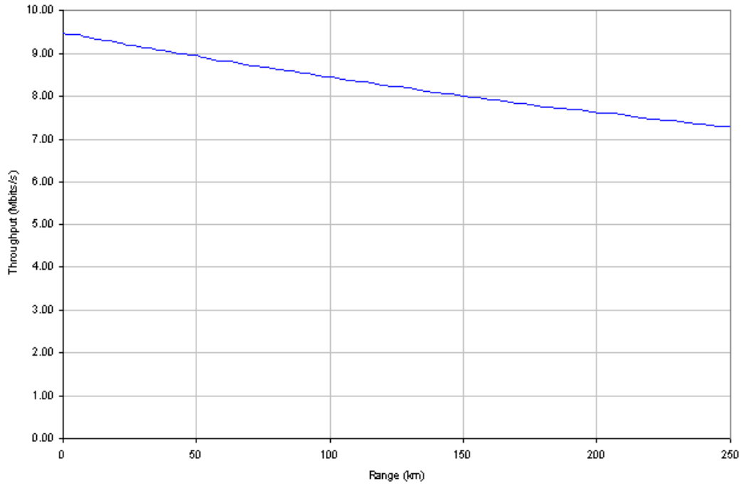
Figure 111 - QPSK 0.50 Single Payload
