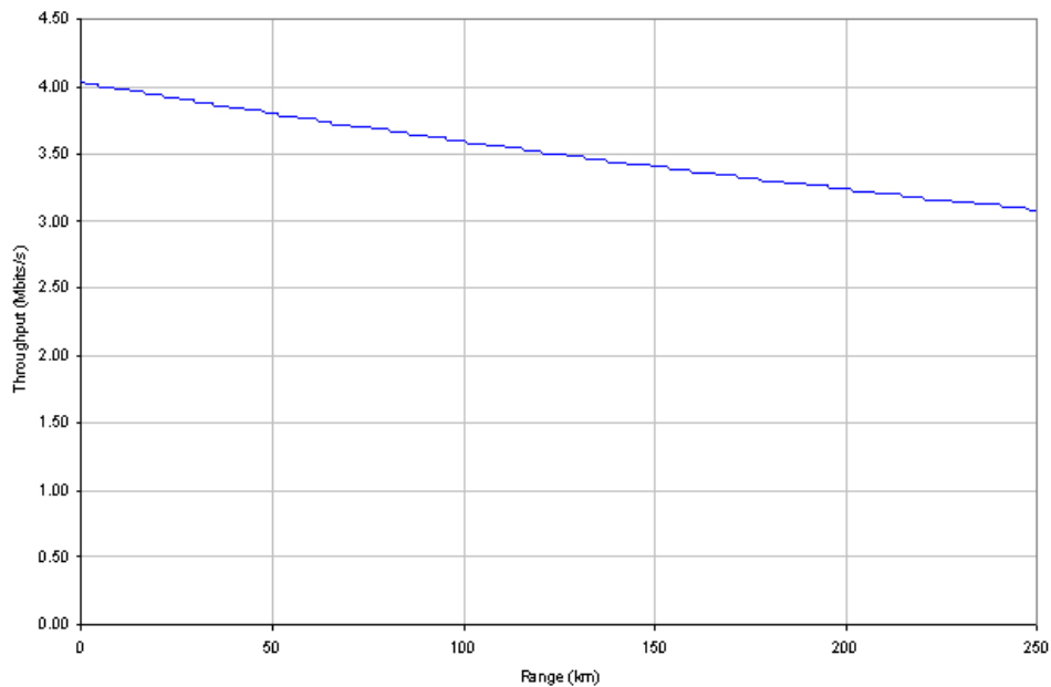
Figure 110 - BPSK 0.50 Single Payload
