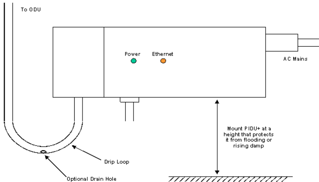
Figure 23 – PTP 500 Series PIDU Plus Drip Loop Configuration
