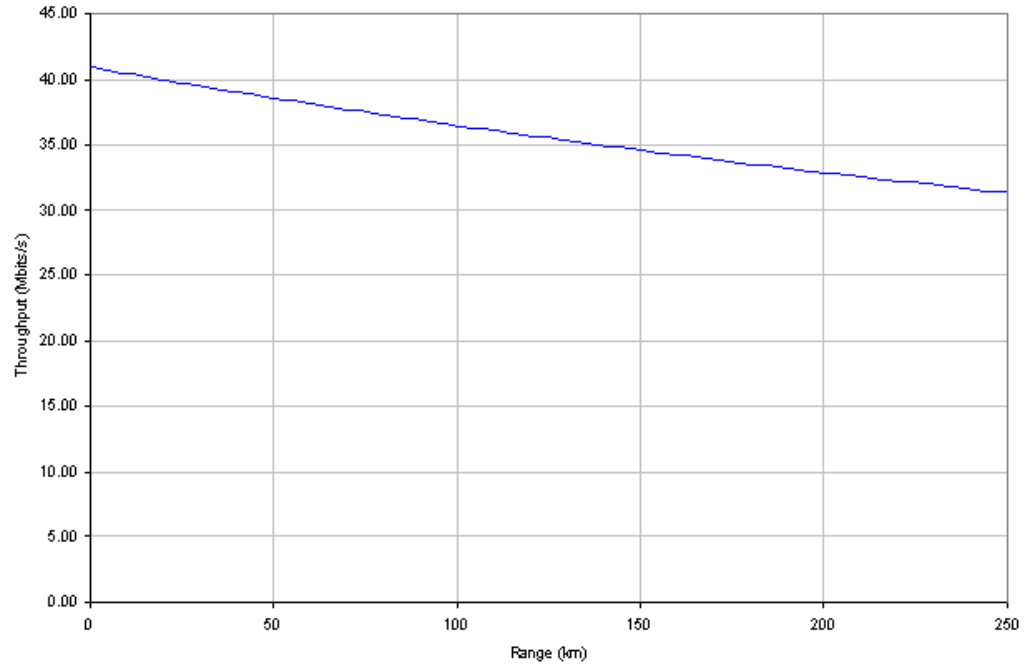
Figure 115 - 64 QAM 0.67 Single Payload
