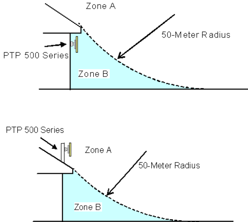
Figure 92 - ODU mounted in Zones A & B
