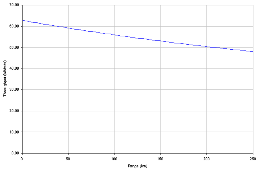
Figure 120 - 16 QAM 0.75 Dual Payload
