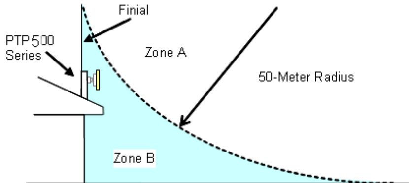
Figure 93 - Showing how the use of a Finial enables the ODU to be mounted inside Zone B
