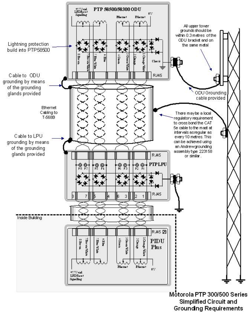
Figure 97 - Simplified Circuit Diagram
