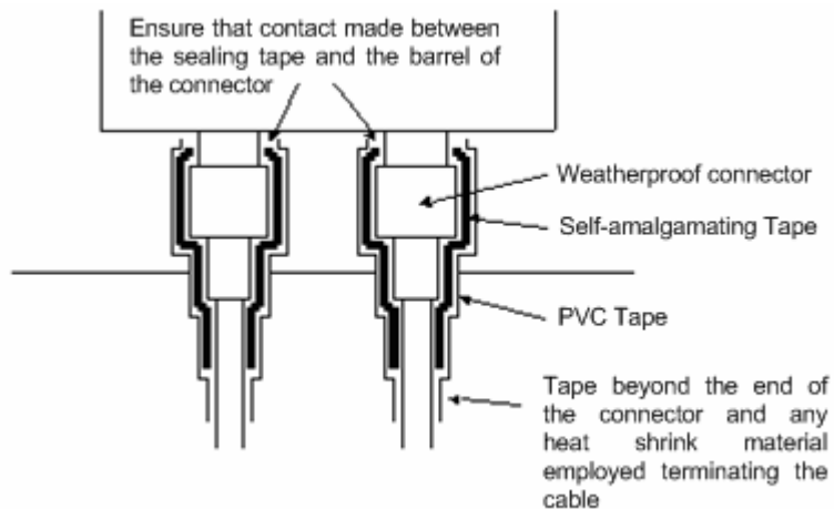
Figure 106 - Weatherproofing the Antenna Connections
