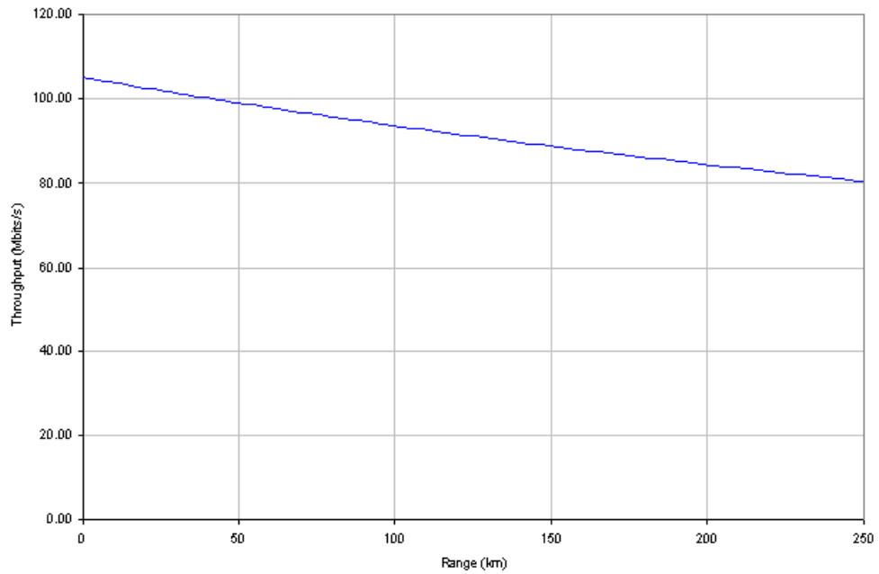
Figure 122 - 64 QAM 0.83 Dual Payload
