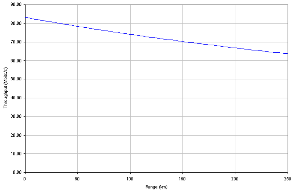
Figure 121 - 64 QAM 0.67 Dual Payload
