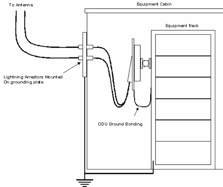
Figure 108 - Lightning Arrester Mounting
