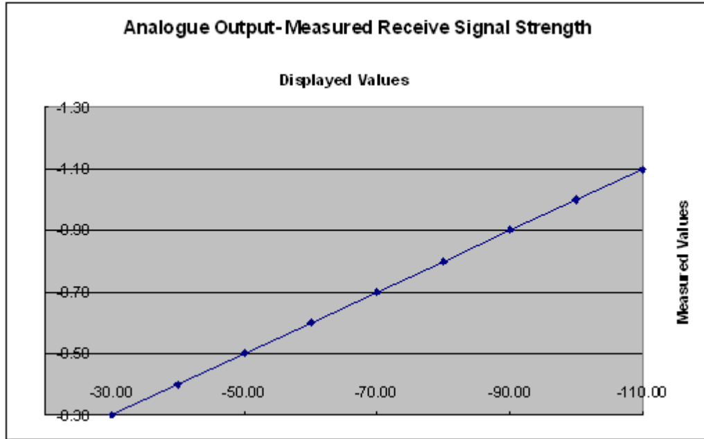
Figure 24 - Using DVM For Alignment
