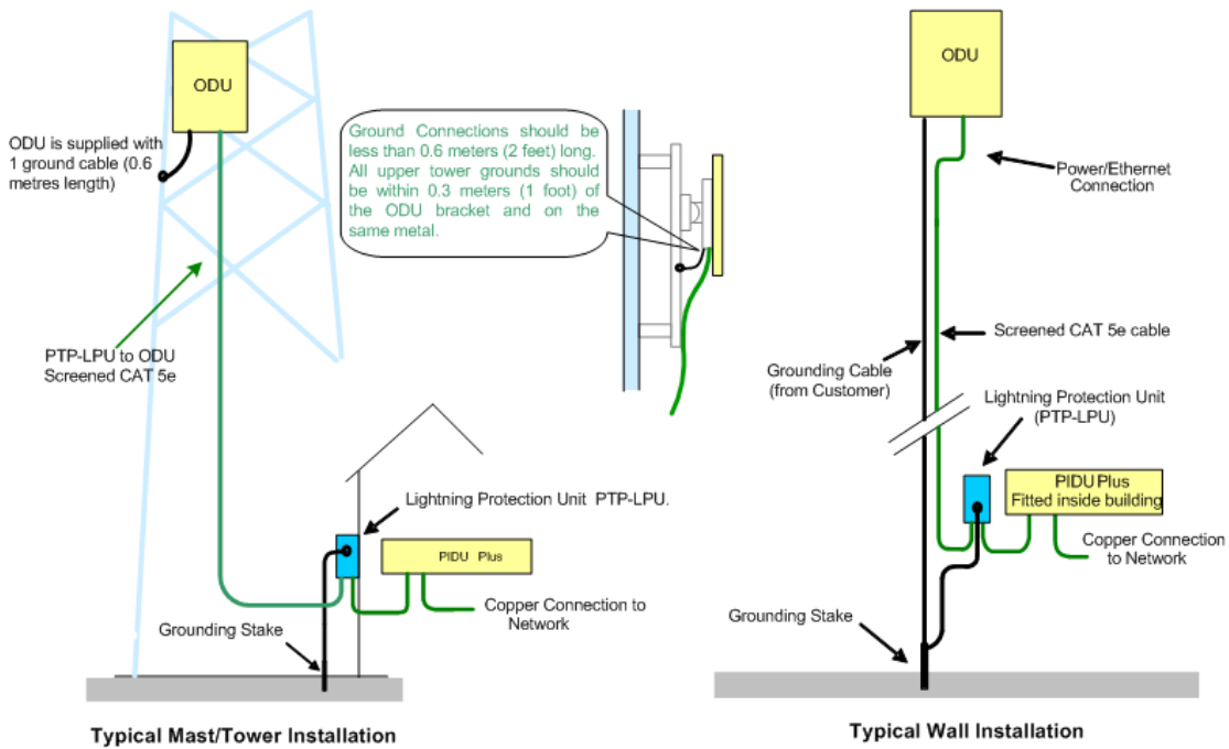
Figure 94 - Diagrammatically Showing Typical Mast and Wall Installations
