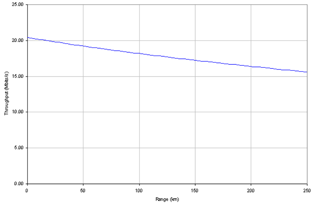
Figure 117 – QPSK 0.50 Dual Payload
