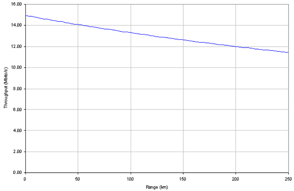
Figure 112 - QPSK 0.75 Single Payload
