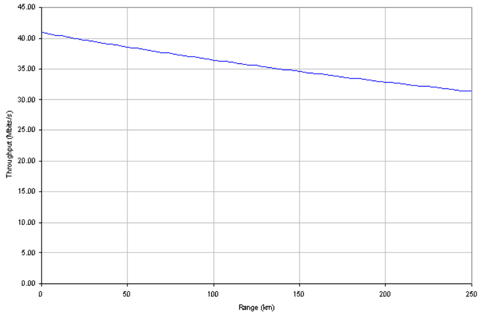
Figure 119 - 16 QAM 0.50 Dual Payload
