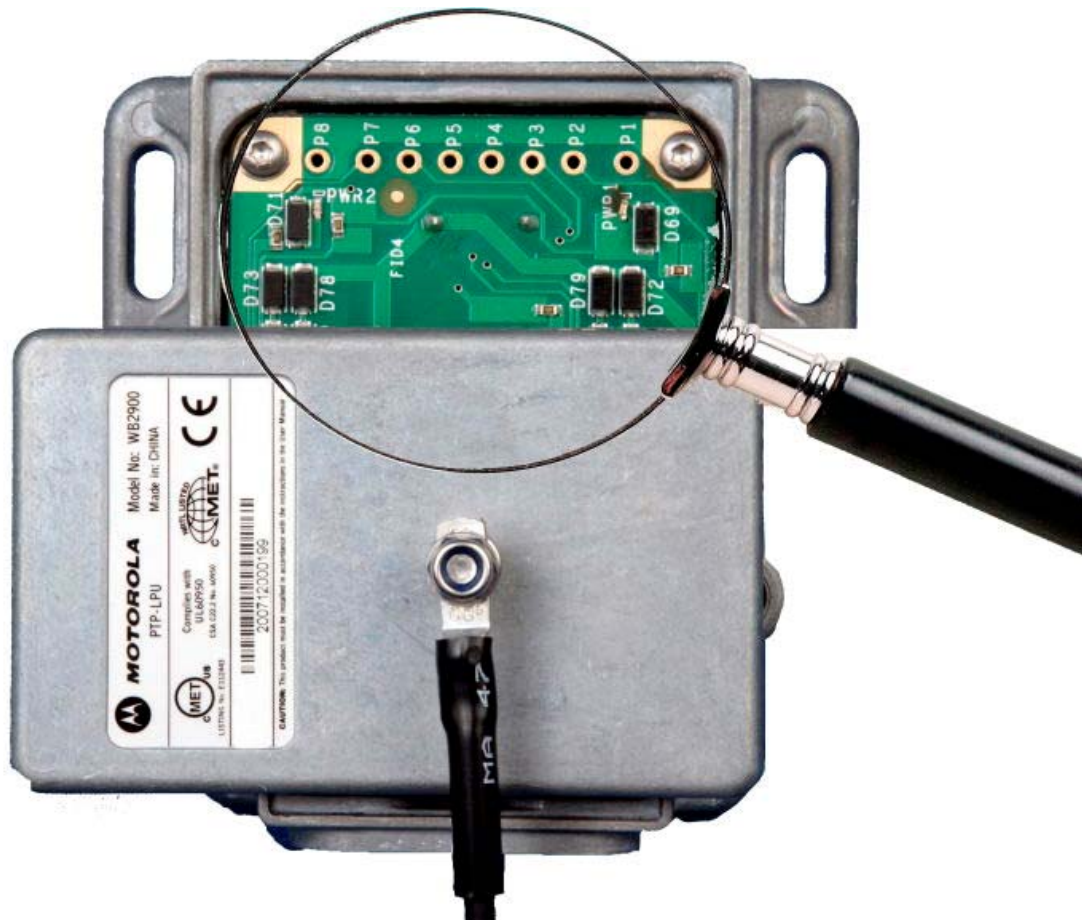
Figure 98 - PTP LPU test Points
