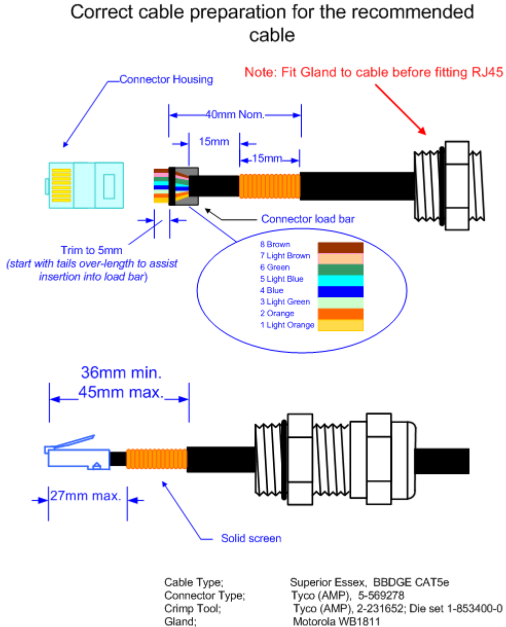
Figure 16 - Correct Cable Preparation for the Recommended Cable
