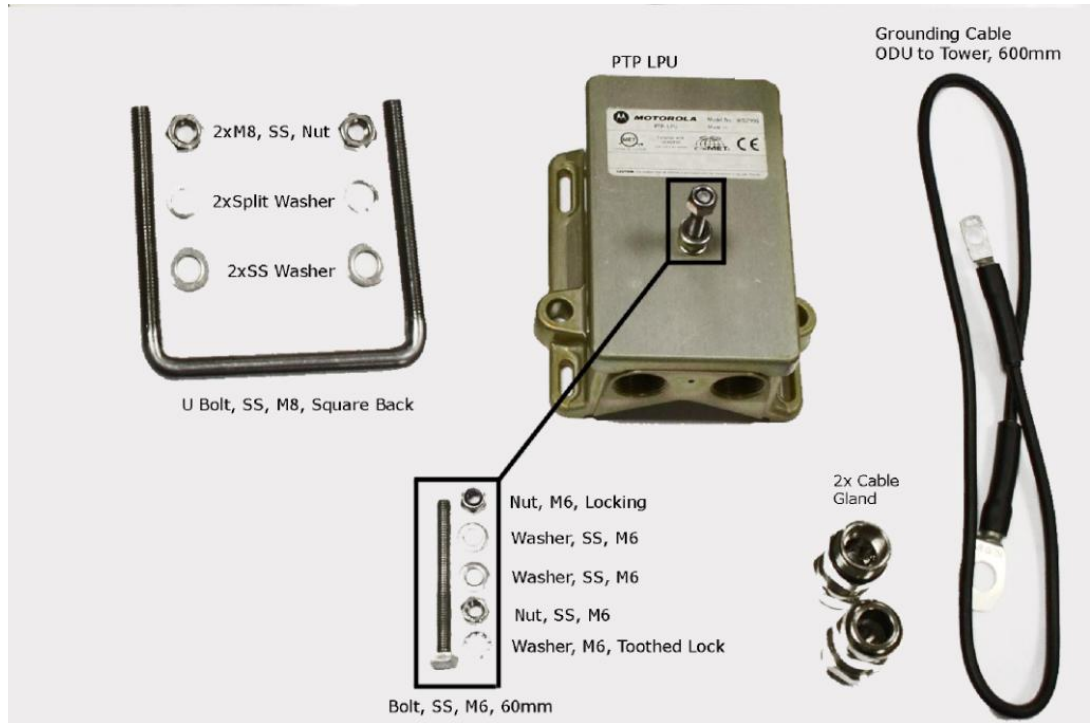
Figure 96 - PTP 500 Series LPU Kit
