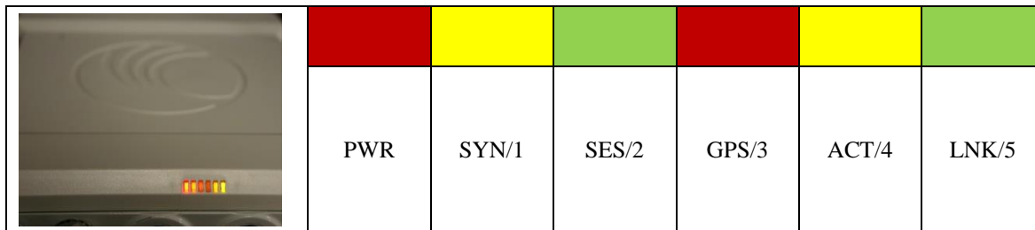
Figure 5 AP diagnostic LEDs, viewed from unit front
