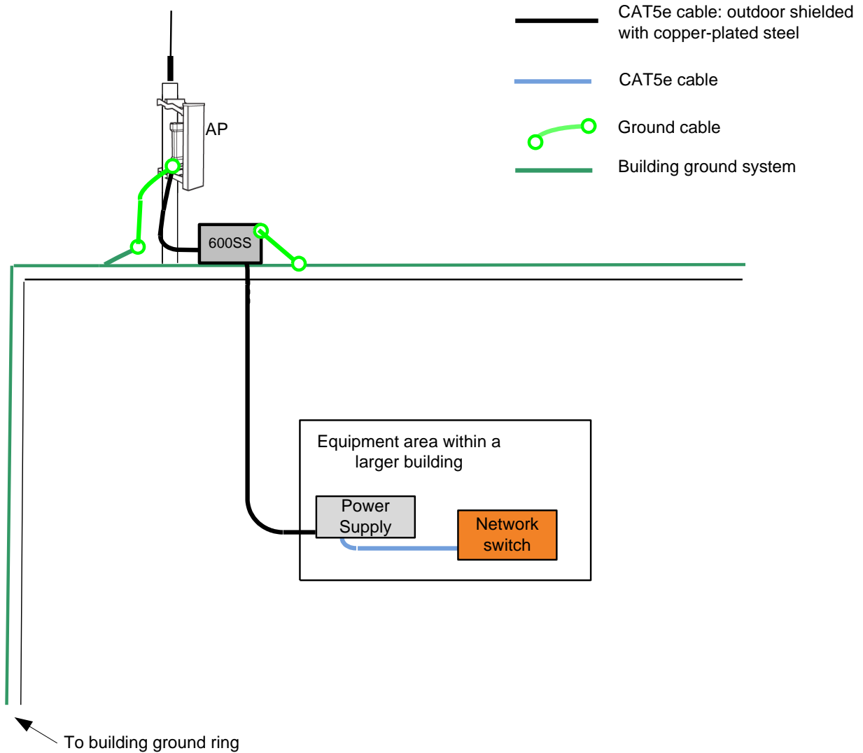
Figure 21 Grounding and lightning protection inside high building
